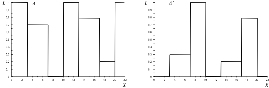
(a) Discrete signal A as an L -Fuzzy set (b) Negation A' of the discrete signal A
