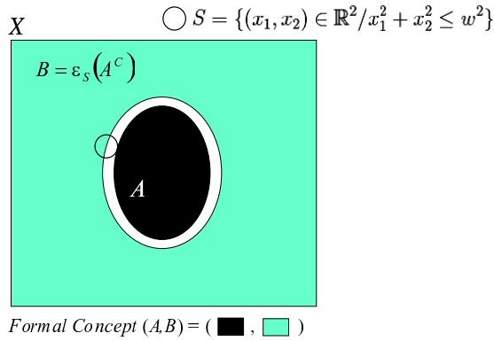
Fig. 1. A formal concept of the context (\mathbb{R}^2, \mathbb{R}^2, R_S^c) .
