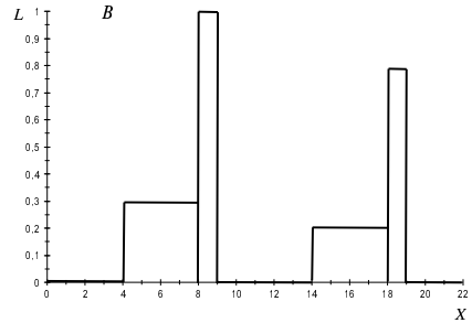
(c) Discrete signal B = \varepsilon_S(A')
