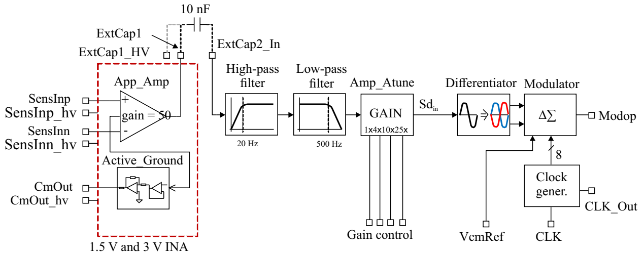
Fig. 1. ASIC level block diagram
