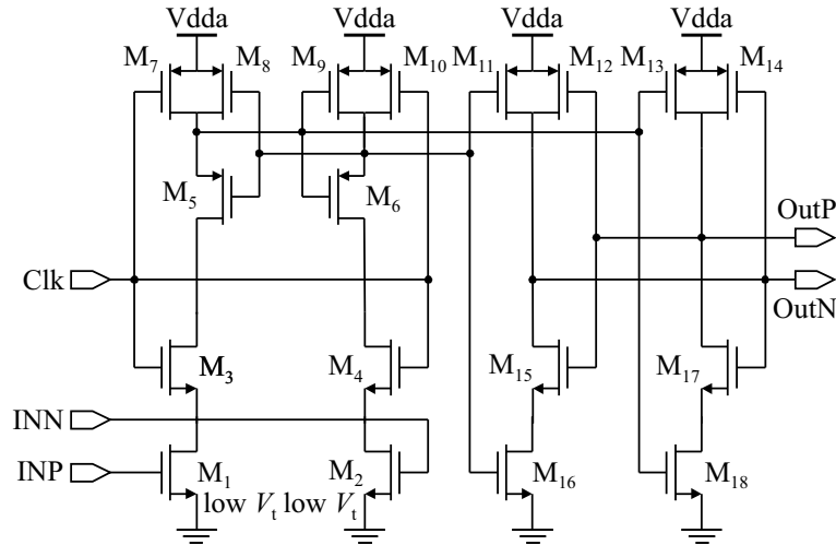
Fig. 5. Circuit diagram of the comparator and latch
