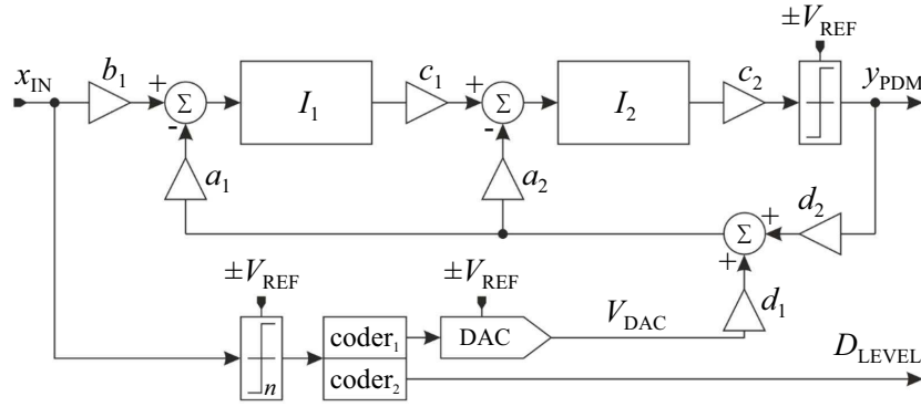
Fig. 3. Circuit diagram of 3rd order \Delta\Sigma modulator
