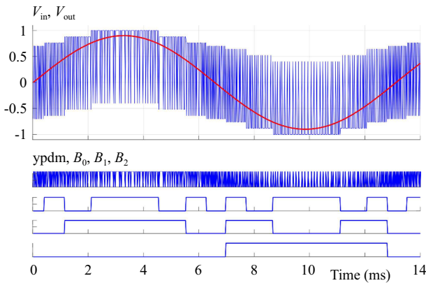
Fig. 4. Waveforms at various nodes of the \Delta\Sigma modulator
