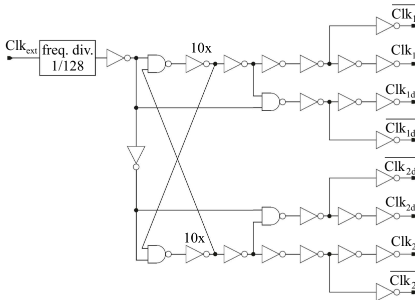
Fig. 6. Non-overlapping clock generator
