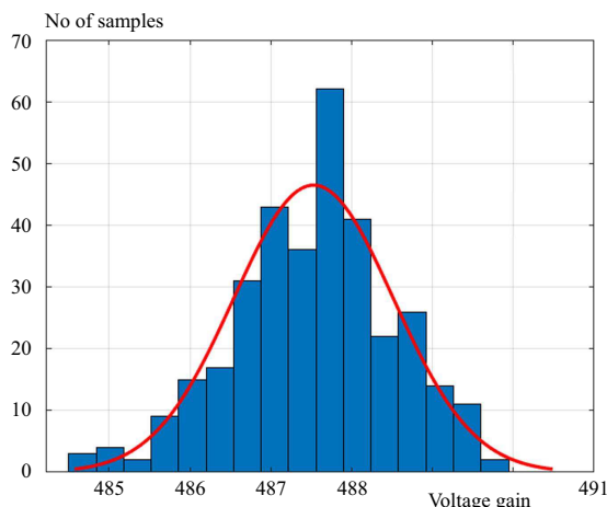
Fig. 8. DC transfer Monte Carlo statistical analysis
