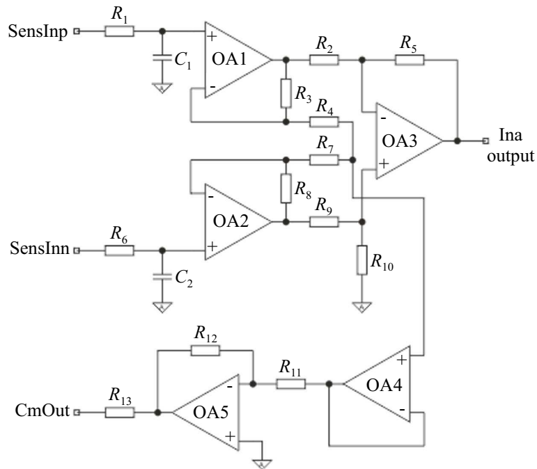
Fig. 2. Circuit diagram of the INA include active ground part
