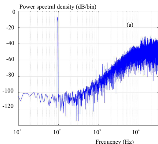
Fig. 9. Delta-sigma modulator measurement results, (a) – power spectral density, and (b) – dynamic range
