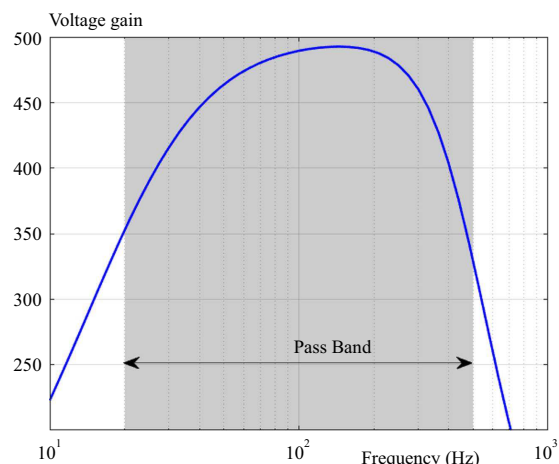
Fig. 7. Measured bandpass characteristic
