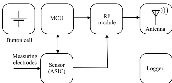
Fig. 11. System architecture
