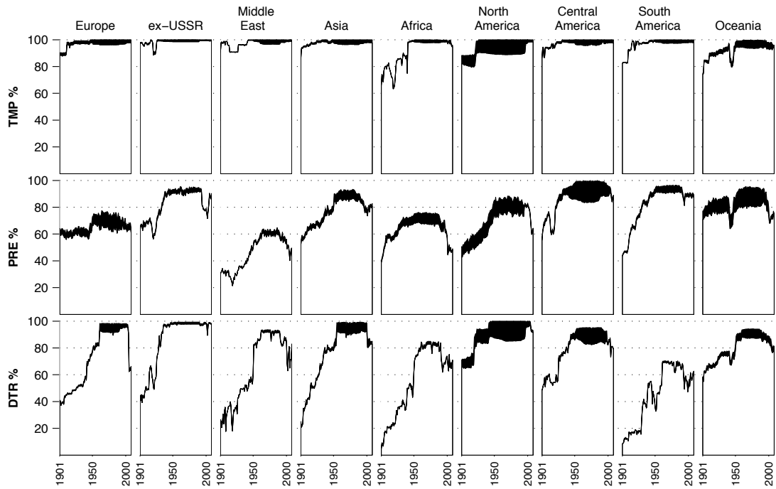
Figure 5: The percentage of half-degree land cells, for the three primary variables (TMP, PRE and DTR) containing stations with valid values (black) or within the CDD of those stations (white). Data are monthly, smoothed with a Gaussian-weighted filter (width = 13).
