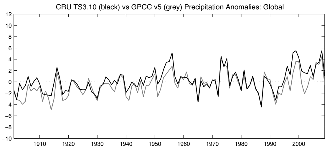
Figure 10: Hemispheric and global comparisons between CRU TS3.10 (black lines) and GPCC v5 (grey lines) for annual total precipitation percentage anomalies, 1901 - 2009. The base period is 1961-90.
