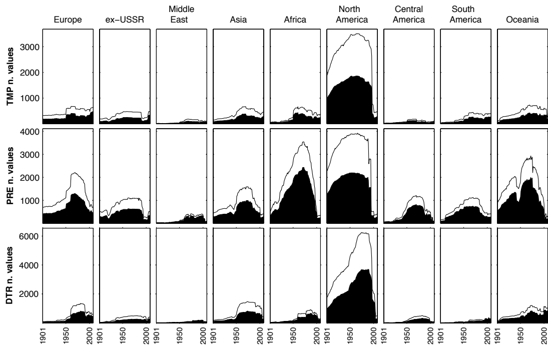
Figure 4: The number of data values per month, for the three primary variables (TMP, PRE and DTR) actually used (shaded) and the total in the databases (top line). The monthly numbers are smoothed with a Gaussian-weighted filter (width = 13). These values may be used as a proxy for station numbers, since the incidence of potentially-duplicate stations (based on spatial metadata) is low (about 1% for TMP, 2.3% for DTR and 0.6% for PRE).
