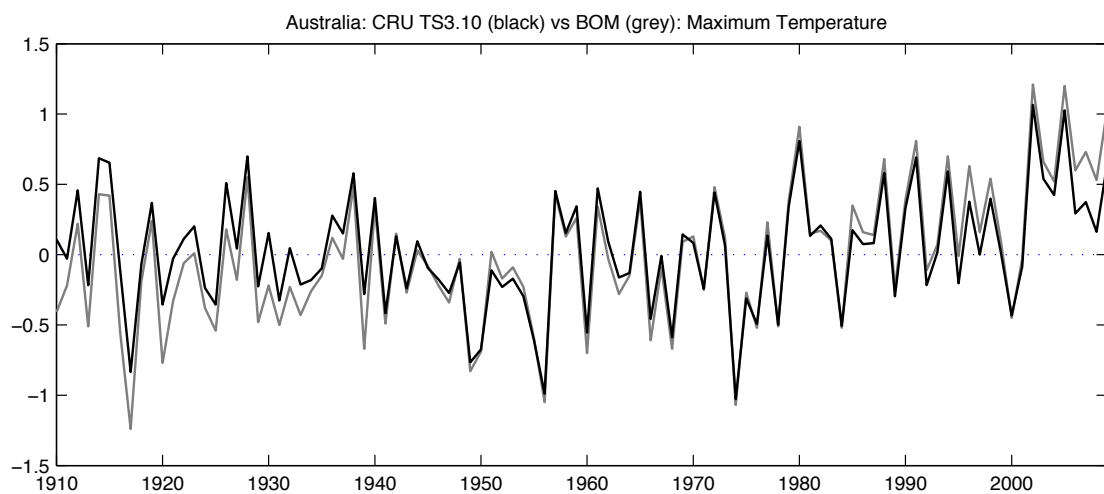
Figure 8: Comparisons between CRU TS3.10 (black) and BoM (grey) for mean, minimum and maximum annual temperature anomalies ( ^{\circ}\text{C} ) for Australia, 1910-2009. The base period is 1961-90.
