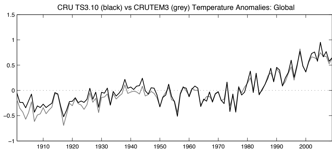
Figure 9: Hemispheric and global comparisons between CRU TS3.10 (black lines) and CRUTEM3 (grey lines) for annual temperature anomalies ( ^{\circ}\text{C} ), 1901 - 2009. The base period is 1961-90.
