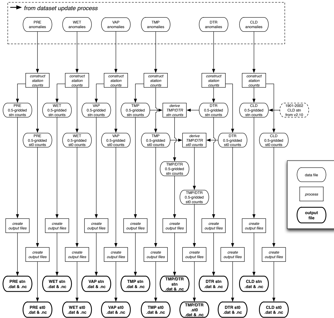
Figure 3: Station Counts Gridding Process. Showing the process by which the station count files are produced as part of the main dataset update process.
