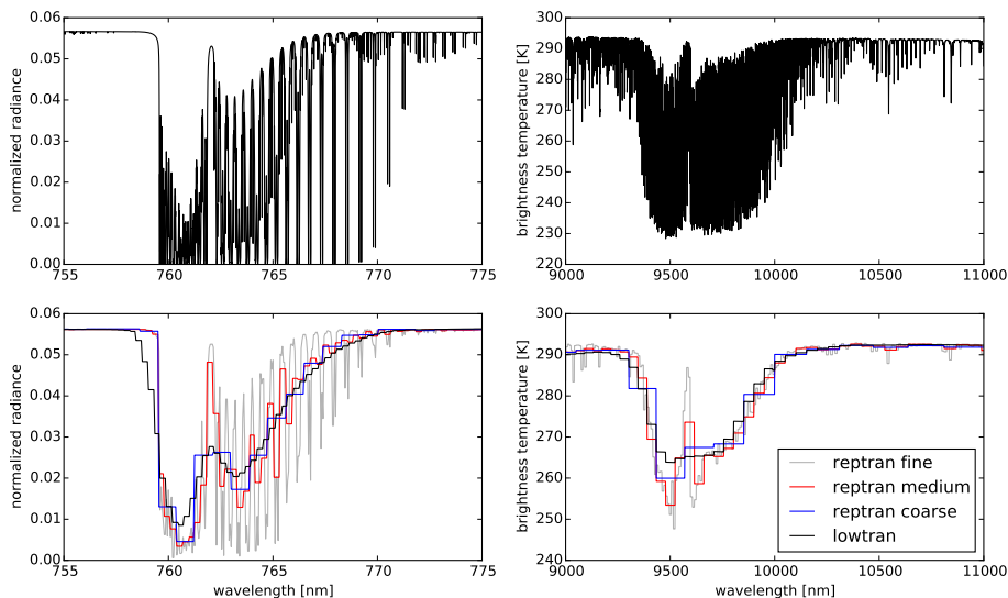
Figure 2. Nadir top of the atmosphere radiance in the oxygen-A band around 760 nm (left) and in the IR window region (right) for the midlatitude-summer atmosphere of Anderson et al. (1986). All calculations were performed with the MYSTIC solver using the “absorption lines importance sampling” method (Emde et al., 2011). (Top) High spectral resolution calculation, based on line-by-line absorption cross sections calculated using ARTS (Eriksson et al., 2011); (bottom) pseudo-spectral calculations using the representative wavelengths band parameterizations ( reptran ) with different resolutions and lowtran . For comparison see also Fig. 3 in Mayer and Kylling (2005) which shows transmittances for genIn2 line-by-line calculations and lowtran for the same spectral regions.
