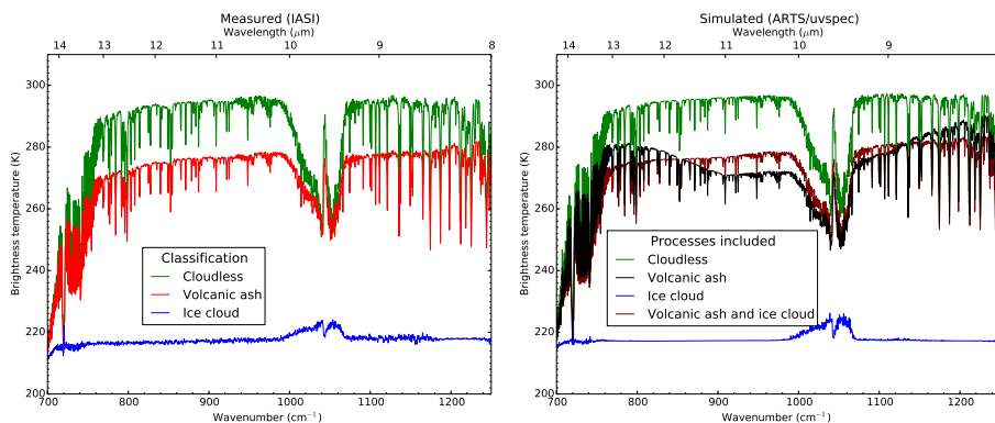
Figure 8. (Left plot) Brightness temperature spectra for different locations as measured by IASI on 15 February 2014, 02:33 UTC, during the Mt. Kelud, Indonesia, eruption. Tentative classification of the spectra is given in the legend. See text for details. (Right plot) Simulated brightness temperature spectra using ARTS/ uvspec . The atmospheric processes included in the simulations are given in the legend.
