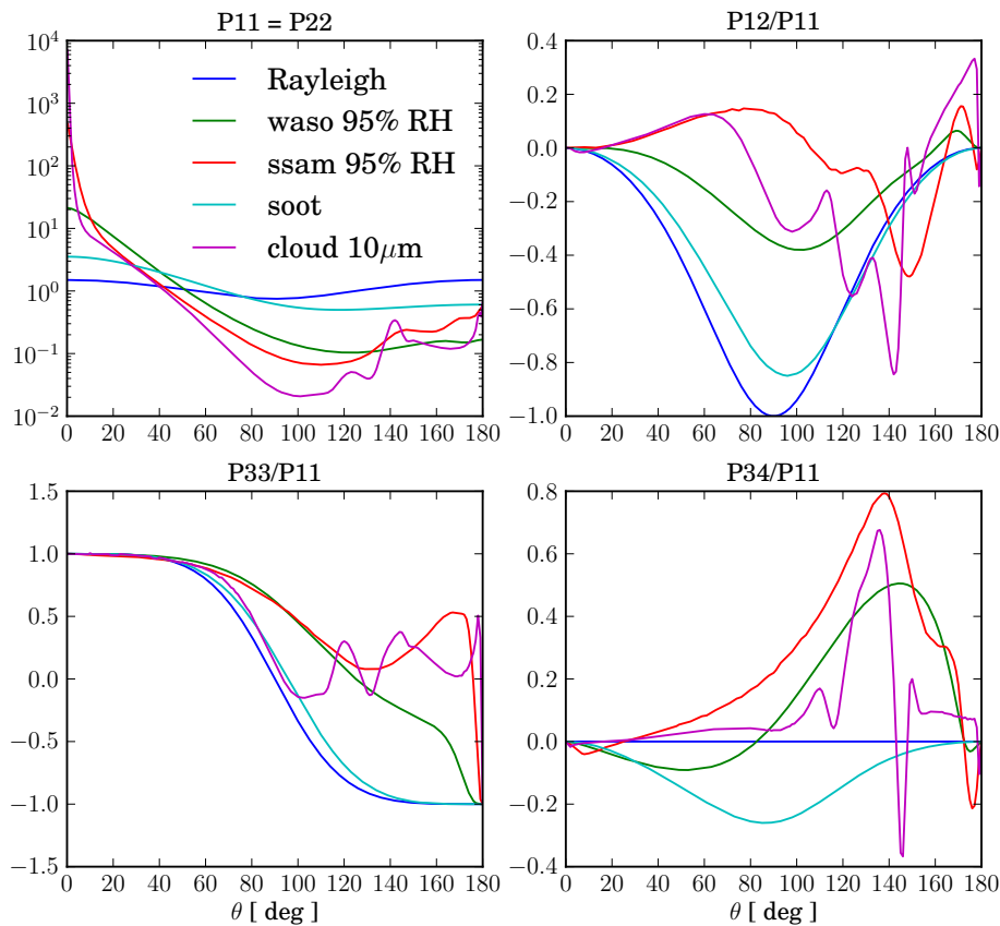
Figure 3. Phase matrix elements for the basic OPAC aerosol types “water soluble” ( waso ), “sea salt accumulated mode” ( ssam ), and soot , for a water cloud with a droplet effective radius of 10\mu\text{m} , and for Rayleigh scattering (with \delta = 0 ) at a wavelength of 350\text{nm} . \theta is the scattering angle, i.e. the angle between incoming and scattered directions.
