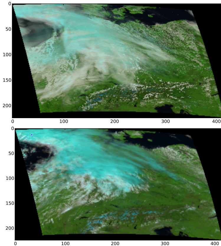
Figure 9. Top: Simulation of MSG-SEVIRI image. False color composite, where red corresponds to the 1.6\ \mu\text{m} channel, green to 0.8\ \mu\text{m} and blue to 0.6\ \mu\text{m} . The simulation was performed using the disort solver with input data from the operational COSMO-DE forecast for the 15 July 2012, 12:00 UTC. The axes correspond to SEVIRI pixel. Bottom: Corresponding SEVIRI image.
