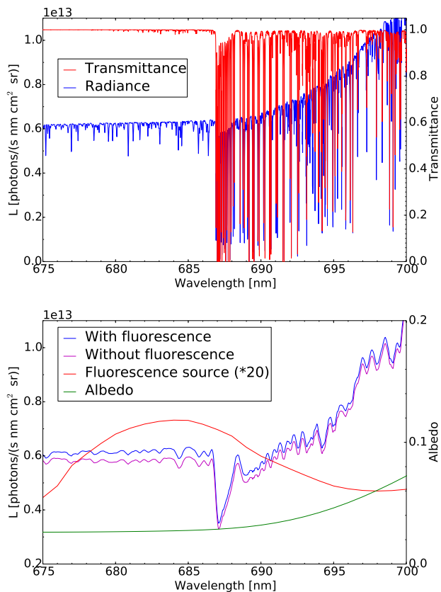
Figure 7. (Upper plot) The transmittance from ARTS output and radiance from uvspec . (Lower plot) The top of the atmosphere nadir viewing radiance in the O 2 -B band with (blue line) and without (purple line) a surface fluorescence source (red line). The radiances have been convolved with a spectral response function with FWHM of 0.3 nm.
