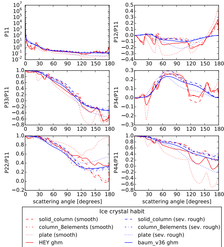
Figure 5. Phase matrix elements of ice crystal distributions with an effective radius of 40\ \mu\text{m} at 550\ \text{nm} wavelength. The red lines correspond to smooth and the blue lines to severely rough crystals, respectively. The individual habits ( solid-column , column-8elements and plate ) are for the parameterization yang2013 , and the general habit mixtures ( ghm ) are for hey including smooth crystals and baum_v36 including severely rough particles.
