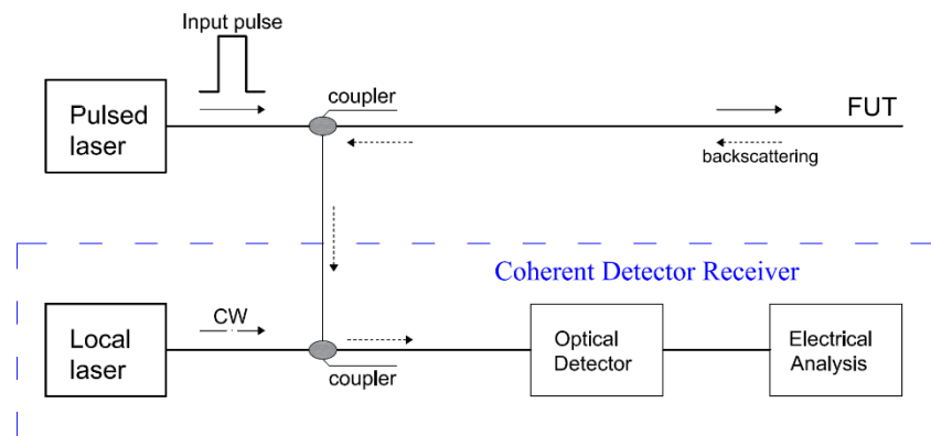
Figure 5. Typical configuration of a BOTDR setup.
