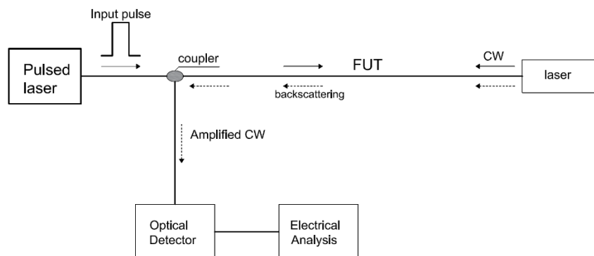
Figure 6. Typical configuration of a BOTDA setup.
