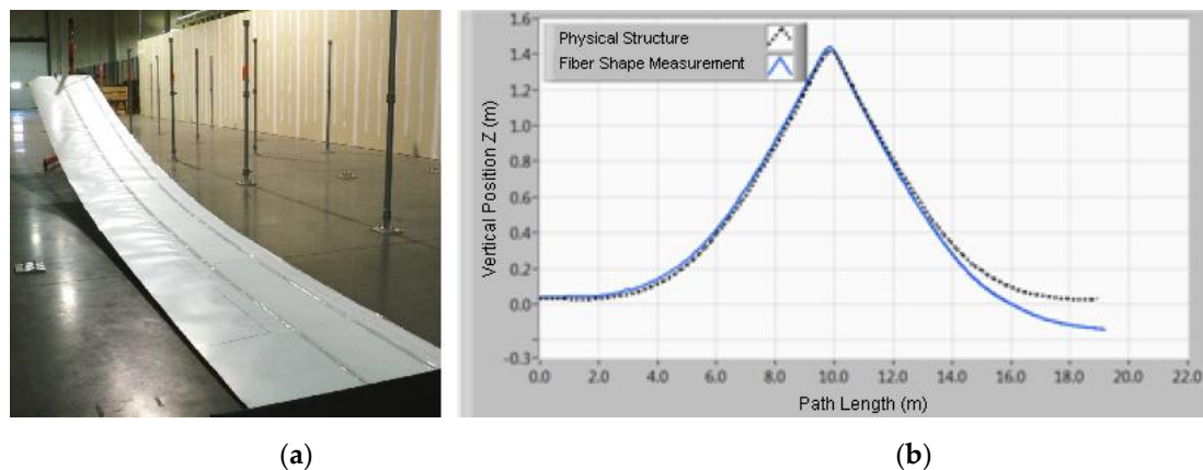
Figure 31. (a) experimental setup; (b) obtained results (adapted from [126]).
