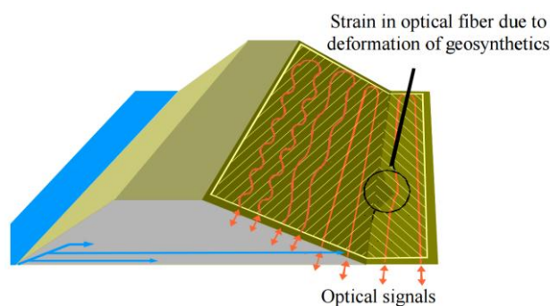
Figure 27. River dike with sensor-based geosynthetics [26].
