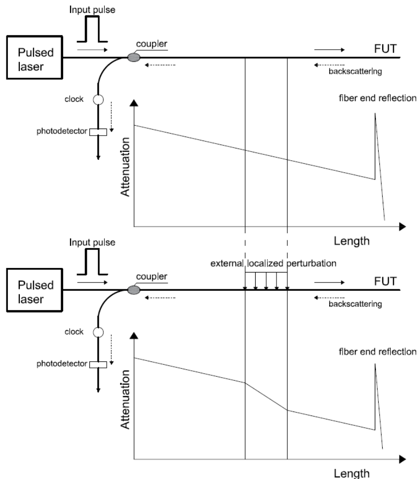
Figure 4. Principle OTDR based on Rayleigh backscattering.
