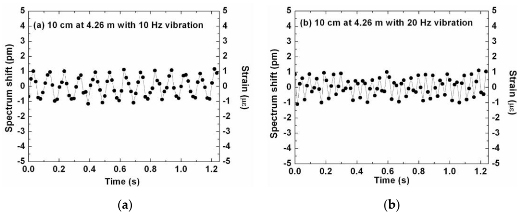
Figure 33. Time-domain Rayleigh backscatter spectrum shift (applied strain) with 10 cm spatial resolution when (a) 10 Hz and (b) 20 Hz sinusoidal voltage is applied to the PZT tube. [142].
