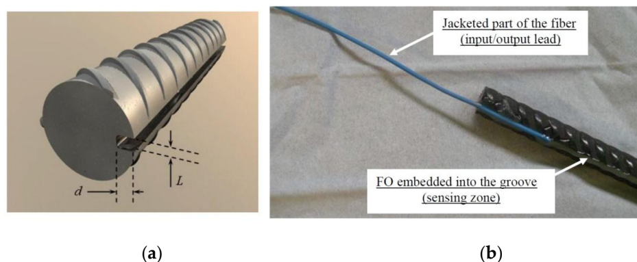
Figure 7. Geometry of the groove in the rebar (a) detail view of the end of the bonded zone (b) [84].
