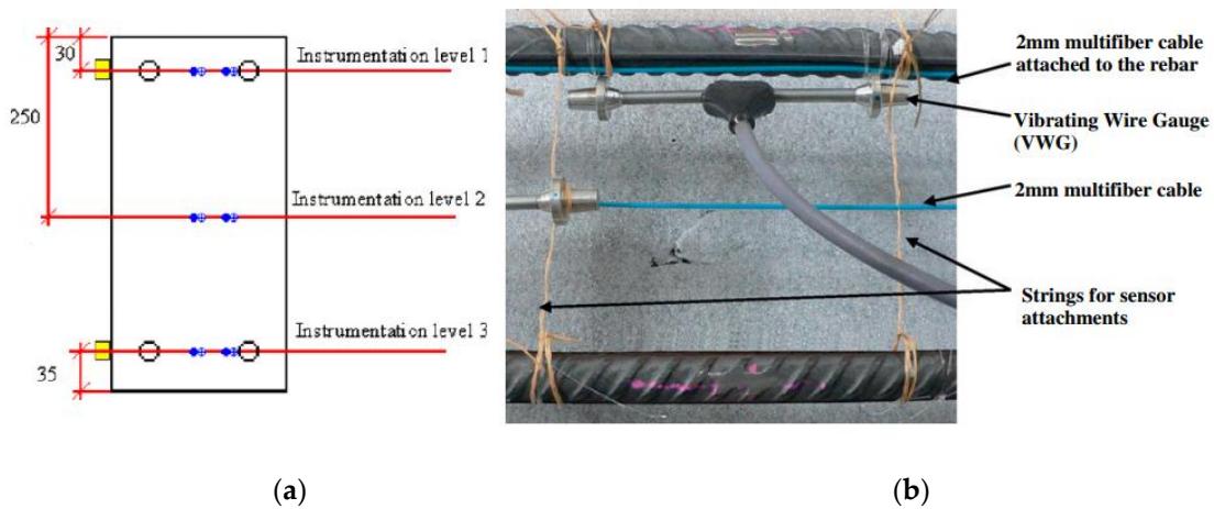
Figure 11. (a) Details of the cross-sectional instrumentation at mid-span of the beam (dimensions in mm); (b) Picture of the instrumented beam before concrete pouring (adapted from [92]).
