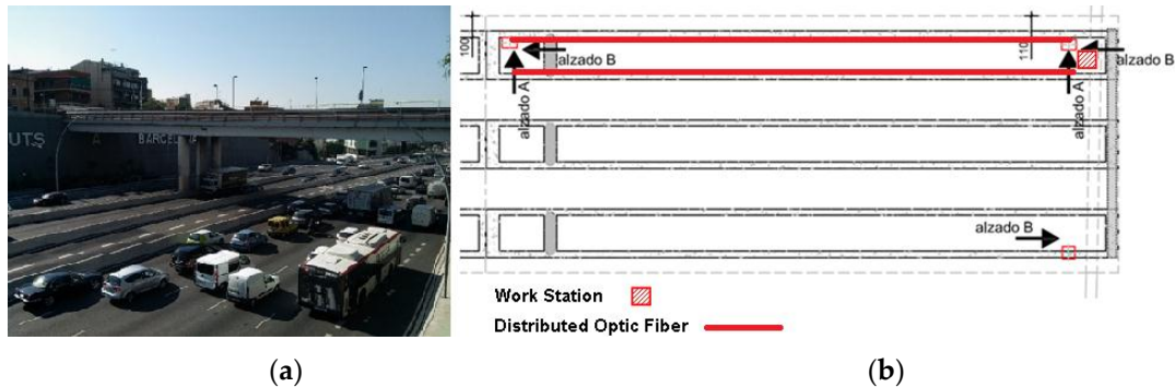
Figure 26. Sarajevo Bridge at Barcelona (a) and general scheme of DOFS monitoring scheme (b) (adapted from [123]).
