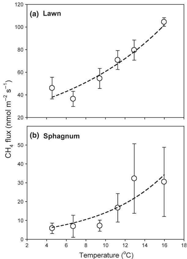
Fig. 3 The relationship between temperature and CH 4 emissions in (a) lawns and (b) Sphagnum interhummocks, the two subunits with the greatest flux rates. Mean fluxes \pm 1 SE are shown (lawn, n = 8 ; Sphagnum , n = 4 ). Exponential equations were fitted to each dataset (dashed lines), and the parameters are presented in Table 1.
