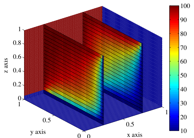
Figure 2: Temperature distribution for a 100.000 mesh.
