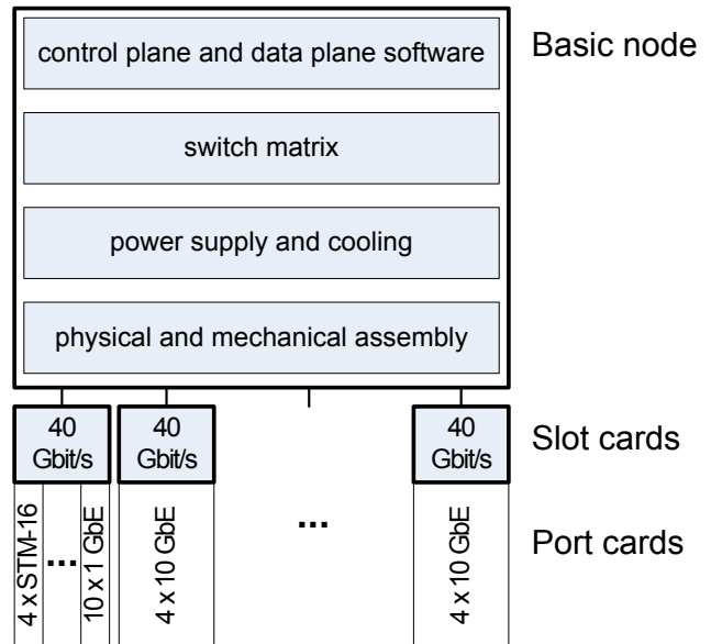
Fig. 1 Simplified IP/MPLS router block model (from [6])
