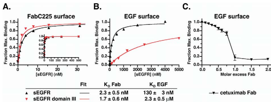
Figure 2. The cetuximab Fab fragment binds to sEGFR and inhibits sEGFR binding to EGF
