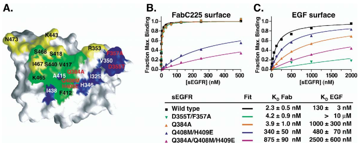
Figure 5. Mutational analysis of cetuximab epitope on sEGFR
