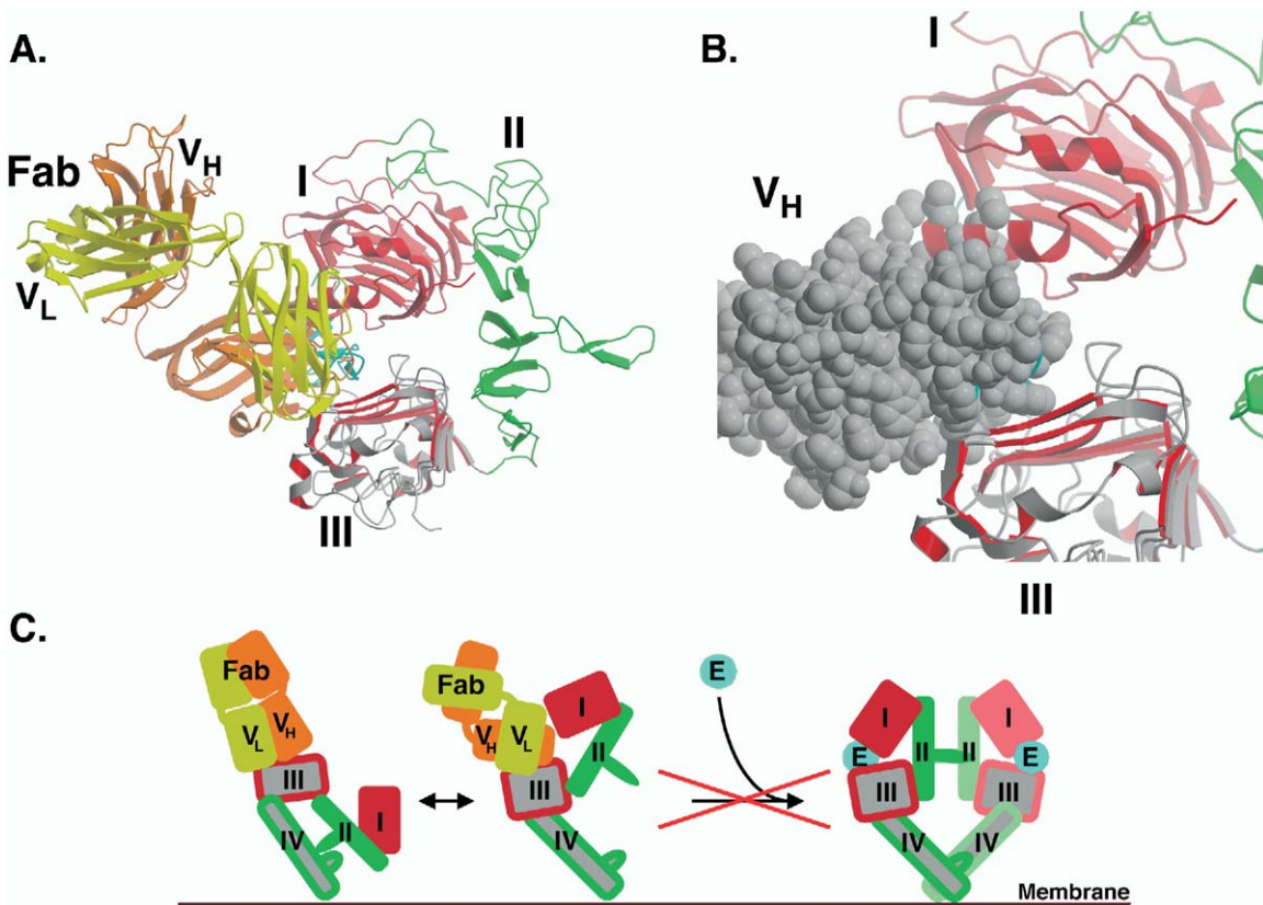
Figure 6. Cetuximab prevents sEGFR from adopting the extended conformation
