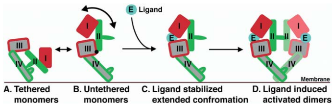
Figure 1. Mechanism of ligand-induced EGFR dimerization
