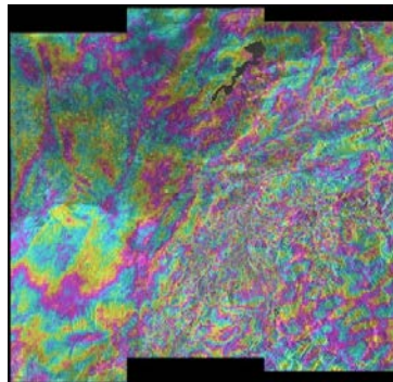
Fig. 5 S1 TOPS differential interferogram as obtained after the spectral diversity co-registration refinement. The phase matches well between bursts and adjacent sub-swaths.
