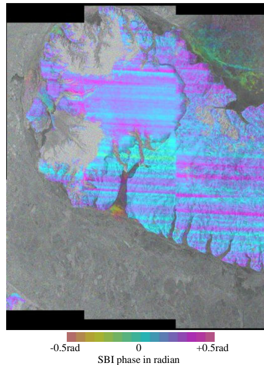
Figure 12 Devon Ice Cap, Canada. Split beam interferometric phase of S1 IWS pair of 20150117 and 20150129 showing “ionospheric azimuth streaking” of the order of 0.5 radian.
