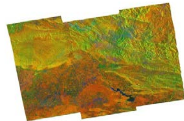
Fig. 6 S1 IWS geo-referenced RGB composite of the coherence (red), the backscatter (green) and the backscatter change (blue).
