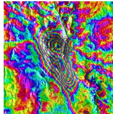
Fig. 7 Co-seismic 6-day S1A – S1B TOPS differential interferogram (ascending orbits, 20160822 – 20160828) over central Italy. The image to the left shows the complex valued differential interferogram, the image in the center the unwrapped and slightly filtered differential interferometric phase (using a cyclic color scale with 6.28 radian per color cycle, i.e. corresponding to the wrapped phase), and the image to the right shows an enlarged section with the main deformation pattern.
