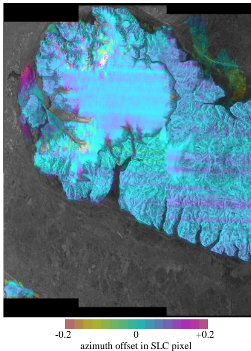
Fig. 11 Devon Ice Cap, Canada. Azimuth offsets between S1 IWS data of 20150117 and 20150129 showing “ionospheric azimuth streaking” of the order of 0.1 SLC pixel.
