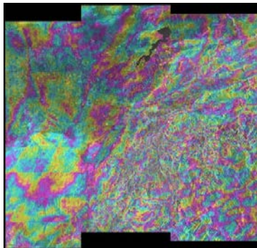
Fig. 4 S1 TOPS differential interferogram after the matching co-registration refinement. Phase jumps are clearly visible between some consecutive bursts.
