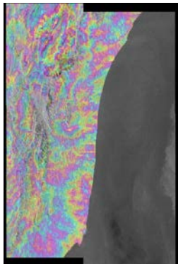
Fig. 7 Co-seismic 6-day S1A – S1B TOPS differential interferogram (ascending orbits, 20160822 – 20160828) over central Italy. The image to the left shows the complex valued differential interferogram, the image in the center the unwrapped and slightly filtered differential interferometric phase (using a cyclic color scale with 6.28 radian per color cycle, i.e. corresponding to the wrapped phase), and the image to the right shows an enlarged section with the main deformation pattern.
