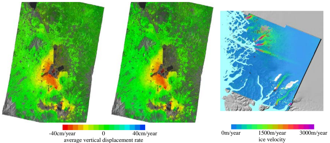
Fig. 8 Average vertical displacement rate derived from a stack of 12 S1 IWS SLC over Mexico City using an SBAS procedure
