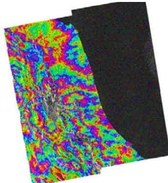
Fig. 7 Co-seismic 6-day S1A – S1B TOPS differential interferogram (ascending orbits, 20160822 – 20160828) over central Italy. The image to the left shows the complex valued differential interferogram, the image in the center the unwrapped and slightly filtered differential interferometric phase (using a cyclic color scale with 6.28 radian per color cycle, i.e. corresponding to the wrapped phase), and the image to the right shows an enlarged section with the main deformation pattern.
