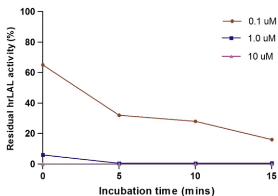
Fig. 4. Lalistat 2 (0.1–10 \mu M) pre-incubated with human recombinant LAL from 0 to 15 min.
