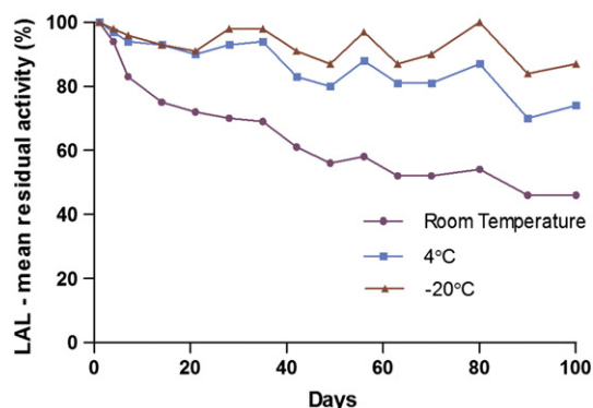
Fig. 5. LAL activity in DBS stored for up to 100 days at room temperature, 4^\circ\text{C} and -20^\circ\text{C} . Results are mean percentage residual activity from three controls.
