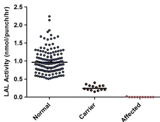
Fig. 6. LAL activity in 140 normal controls, 11 LAL deficient patients and 15 carriers. Limit of detection = 0.02 nmol/punch/h.
