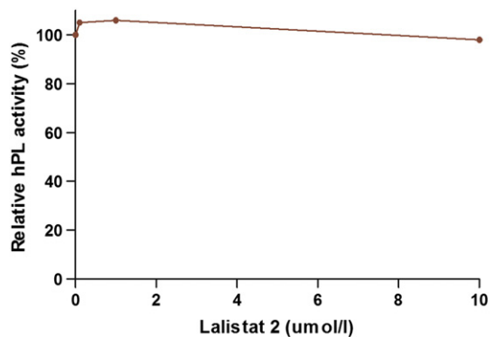
Fig. 2. Inhibitory effect of Lalistat 2 on human pancreatic lipase. Final concentration 6 U/ml. Enzyme pre-incubated with inhibitor for 10 min. Incubation time 2 h.
