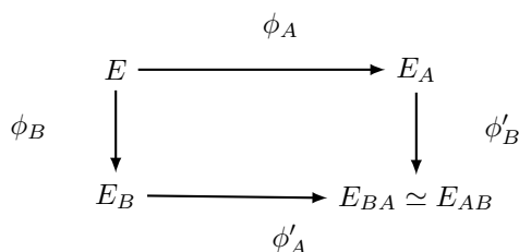
Fig. 1. The SIDH key exchange
