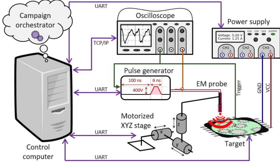
Fig. 7. Campaign setup
