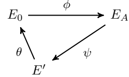
Fig. 6. T has not maximal order.
