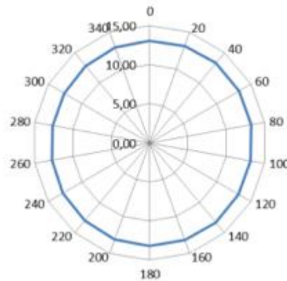
Fig 36. ERP diagram
