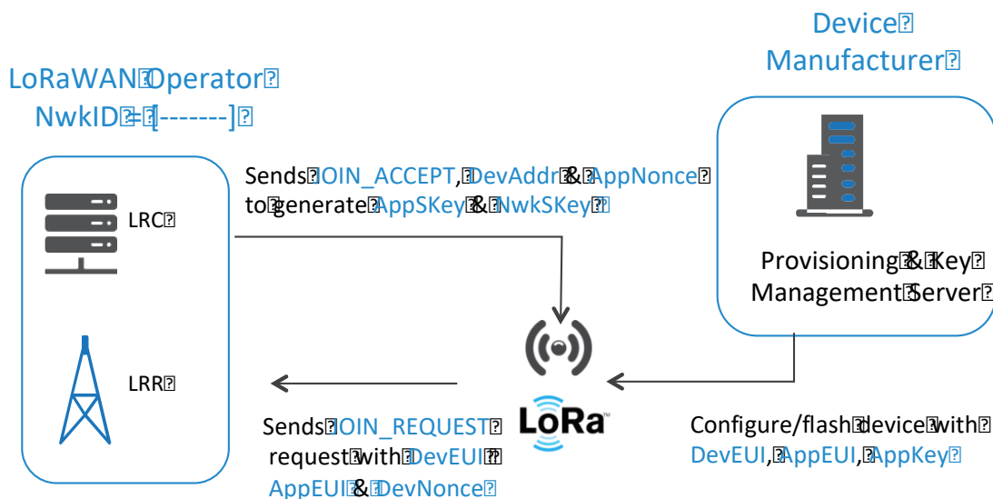
Fig 26. Over-the-air activation
