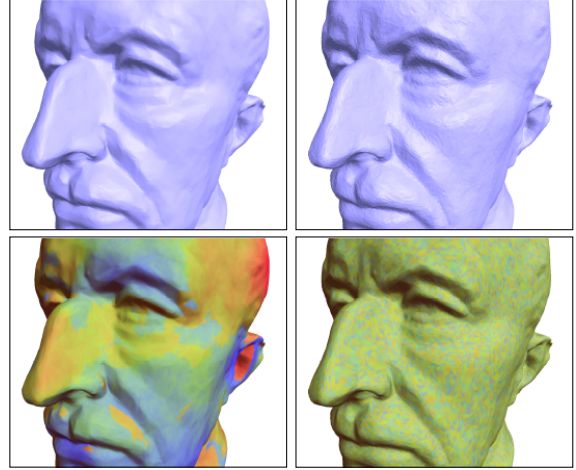
Figure 7: The \delta -coordinates quantization to 5 bits/coordinate (left) introduces low-frequency errors, whereas Cartesian quantization to 11 bits/coordinate (right) introduces noticeable errors. The upper row shows the quantized model, and the bottom figures use color to visualize the corresponding quantization errors. It is recommended to zoom in into the electronic version to see the quantization artifacts.
