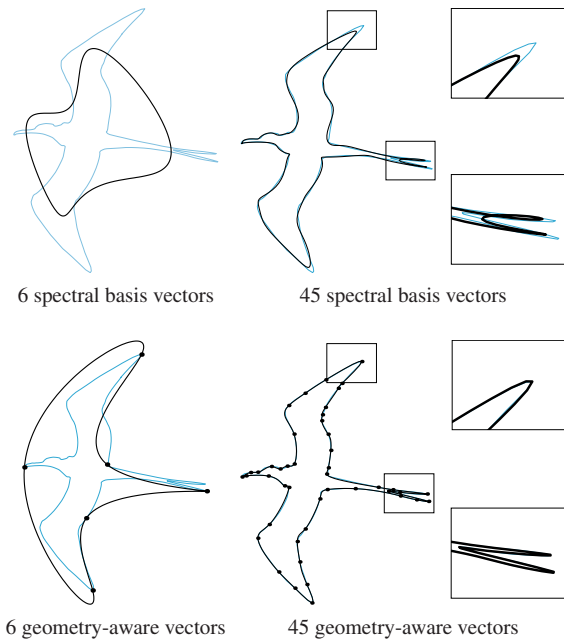
Figure 4: Reconstruction of the swallow curve (simple closed path) using different bases. The top row shows reconstruction using the Laplacian eigenvectors, which are the discrete Fourier basis function in this case. The bottom row displays reconstruction with geometry-aware basis vectors. The reconstructed mesh is shown in black, while the original mesh is tinted in blue. The geometry-aware bases better approximate the features of the shape, on a large as well as on a small scale.
