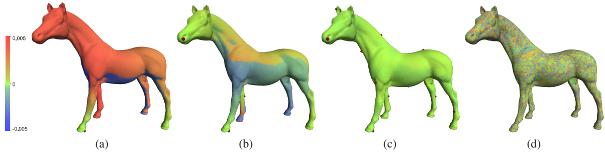
Figure 8: Visualization of the visual error across the mesh surface. The surface was reconstructed from \delta -coordinates quantized to 7 bits/coordinate using 2 anchors (a), 4 anchors (b) and 20 anchors (c). The anchor points are shown as small red spheres. Each vertex v is colored according to its visual error value E_{\text{vis}}(v) . We have also added a sign to these values, so that vertices that move outside of the surface have positive error values (colored by red), and vertices that move inwards have negative error values (colored by blue). In (d), the visual error of direct quantization of the Cartesian coordinates is shown.
