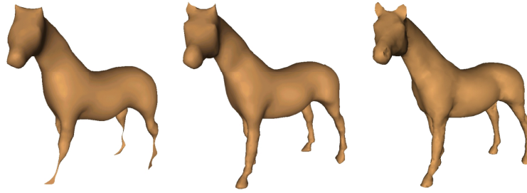
Figure 3: Progressive approximations of the Horse geometry using the eigenvectors of the topological Laplacian [KG00]. The left figure shows an approximation using only a small number of the first eigenvector. When more eigenvectors are added to the approximation, the surface receives more high-frequency detail (middle and right). Data courtesy of Zach Karni.
