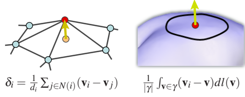
Figure 1: The vector of the differential coordinates at a vertex approximates the local shape characteristics of the surface: the normal direction and the mean curvature.
