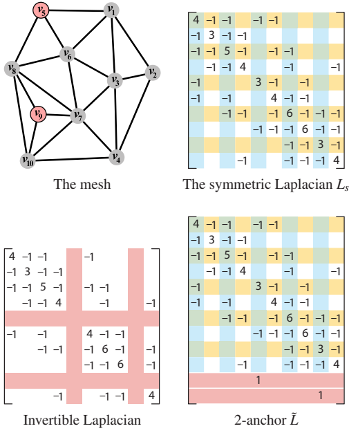
Figure 2: A small example of a triangular mesh and its associated L_s matrix (top right). Second row: a 2-anchor invertible Laplacian and a 2-anchor \tilde{L} matrix. The anchors are denoted in the mesh by red.
