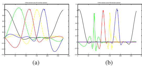
Figure 5: Geometry-aware basis functions on a 1D domain. The mesh here is a simple closed path with 274 vertices. Plot (a) displays the five basis functions corresponding to a set of five anchors; (b) shows the first five basis functions out of a 20-anchor basis.
