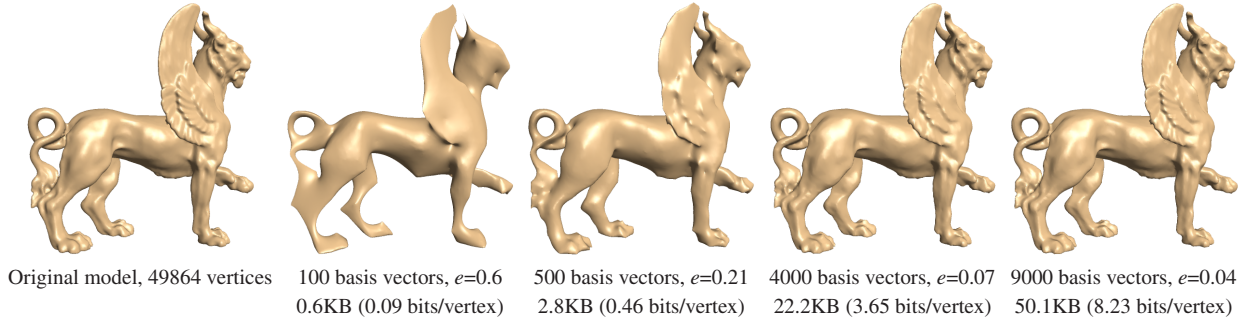
Figure 6: Reconstruction of the Feline model using an increasing number of geometry-aware basis vectors. The sizes of the encoded geometry files are displayed below the models. The letter e denotes the L^2 error value, given in units of 10^{-4} .
