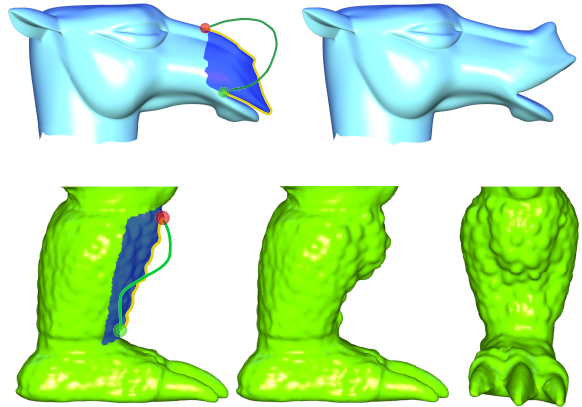
Figure 11: Examples of sketch-based editing of silhouettes [NSACO05]. The sketched curve hints at the new desired shape of the silhouette. By weakly weighting the sketch constraints in the reconstruction process (Eq. 8), the details of the shape are preserved, and the deformation follows the hint of the user.
