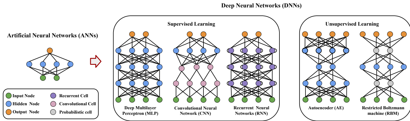
Fig. 2: The visualization of ANNs and DNNs. DNNs have an increasing number of hidden layers embedding the variants of neural nodes and cells. Higher-level feature maps are computed by the deep models. There are five popular DNN architectures for diabetes: DMLP, CNN, RNN, AE, and RBM.
