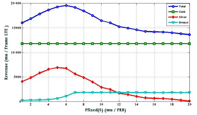
Fig. 3. Mean revenue versus P_{fixed}(S) when using R2P
