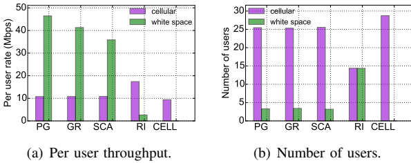
Fig. 3. BC scenario: comparison of algorithms for N = 30 users per cell.
