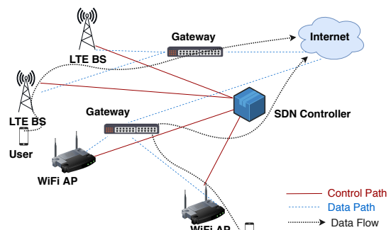
Figure 1: SDN based LTE-WiFi architecture.
