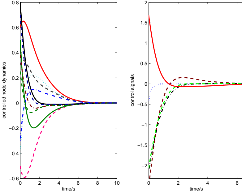
Fig. 2. Evolution of state variables and control signals.
