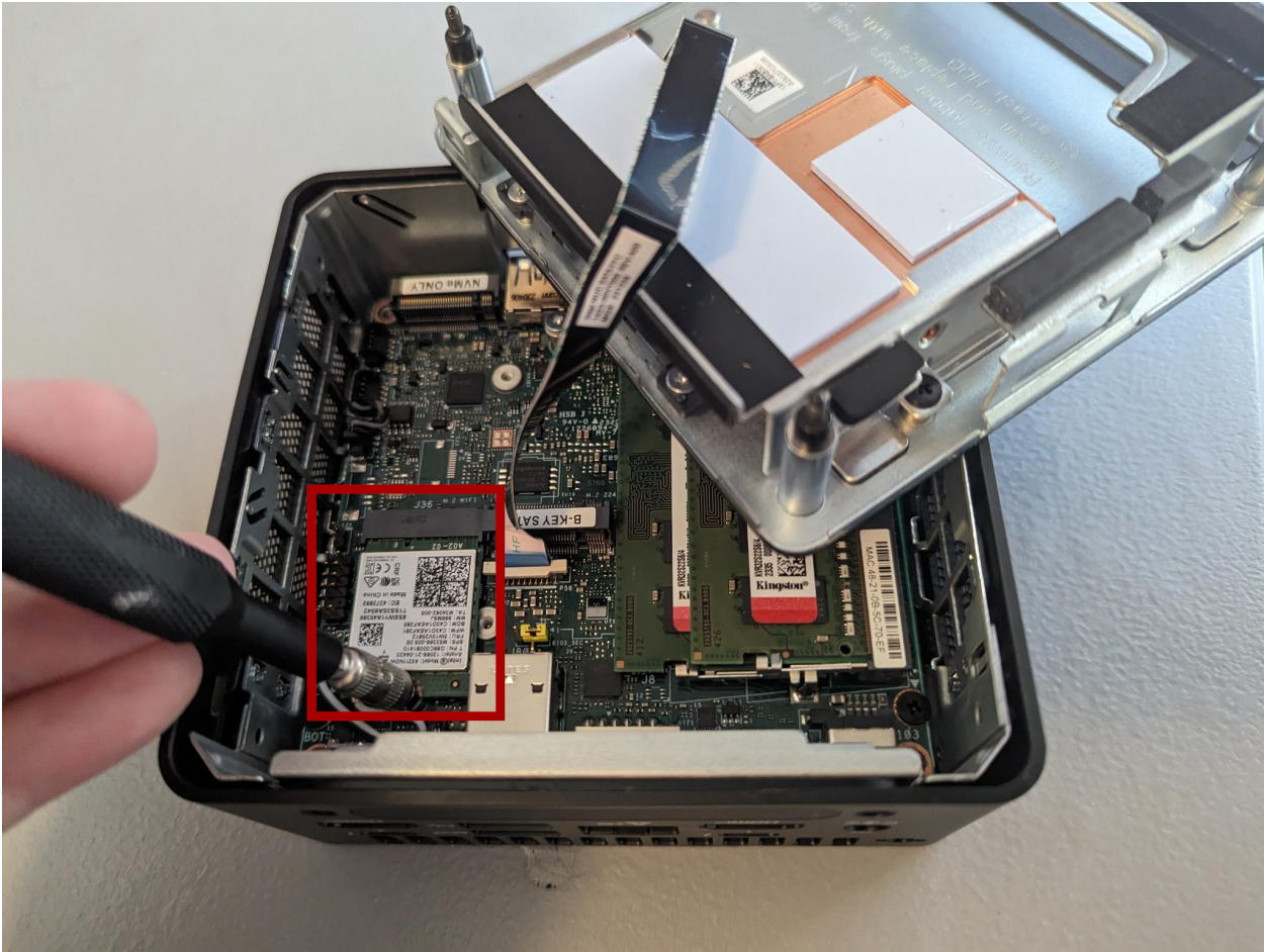
Fig. 1: The location of the wireless card within the NUC13
