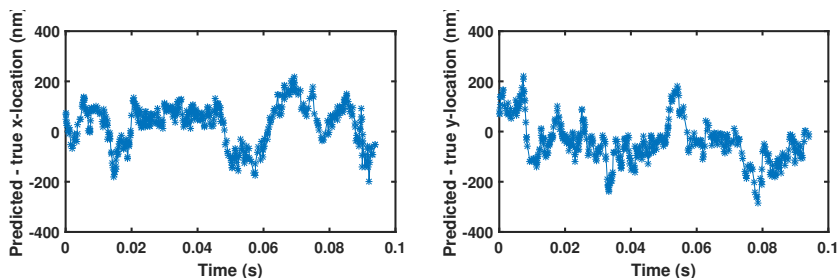
FIG. SM5. Analysis of the error of the predicted locations of the molecule for the Airy measurement model. Shown in the left and right plots are the differences between the means of the distributions of the prediction of the molecule x -locations and the true x -values, and the means of the distributions of the prediction of the molecule y -locations and the true y -values, respectively, for the data sets of Fig. SM3.
