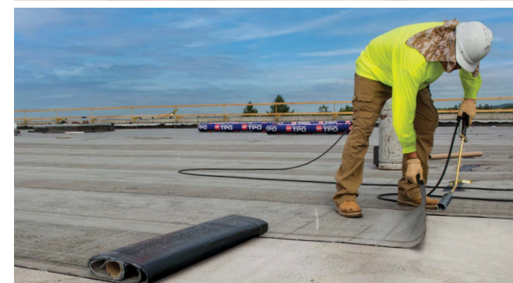
GAF hybrid roof assembly with TPO or PVC fleece-back and asphaltic base sheet
