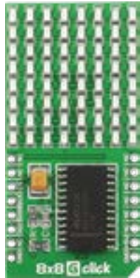
8x8 G Click It features MAX7219 8-digit LED display driver module as well as 64 GREEN LEDs. MSRP - $21 00 MIKROE-1306
