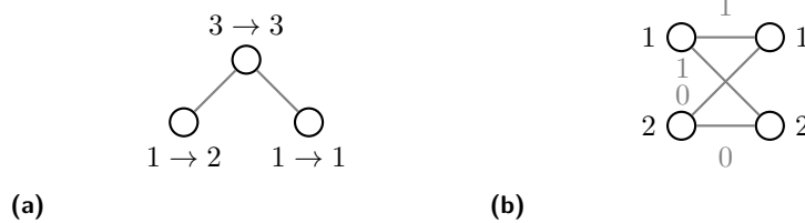
■ Figure 2 Instance of KEMPE DISTANCE on stars (a) and corresponding edge-weighted graph G_{\alpha\beta} (b) for which the approximation algorithm gives a 4-approximate solution. A label a \rightarrow b indicates source color a and target color b for the corresponding vertex.
