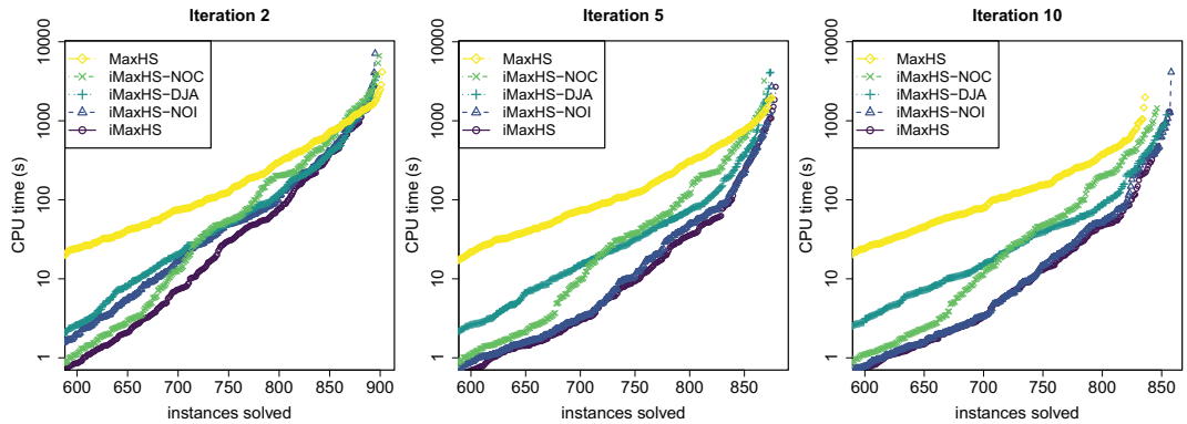
Figure 5 Cactus plots (number of solved instances for a CPU time limit) for different iterations.
