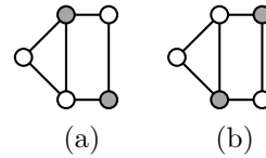
■ Figure 5 The house gadgets used in the IS series. (a) A north-position. (b) A south-position.
