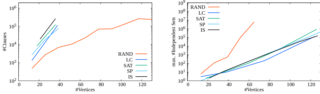
(a) Clauses in the SAT formula with respect to the number of vertices.
