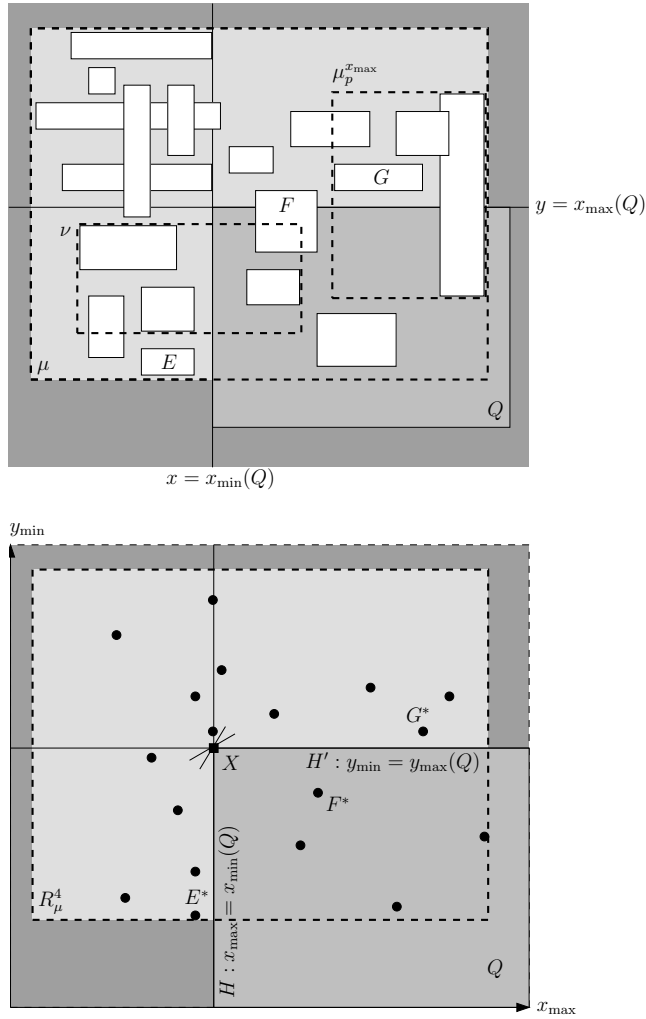
Fig. 2. The proof of Lemma 2, with \mu in the plane (upper figure), and \mu in four-dimensional space (lower figure—the x_{\min} and y_{\max} dimensions are not shown). Note that X = H \cap H' is a two-dimensional hyperplane in four-dimensional space. It contains a two-dimensional facet of the transformation of the query range into four dimensions.
