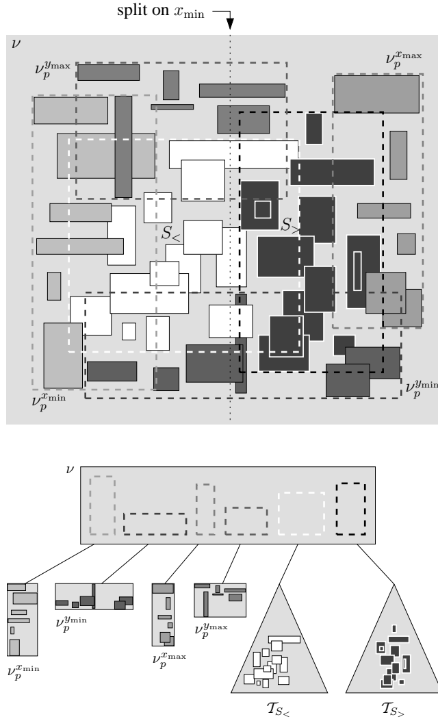
Fig. 1. The construction of an internal node in a pseudo-PR-tree.
