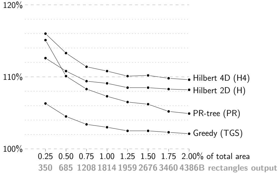
Fig. 13. Query performance for queries with squares of varying size on the Eastern TIGER data. The performance is given as the number of blocks read divided by the output size T/B .
