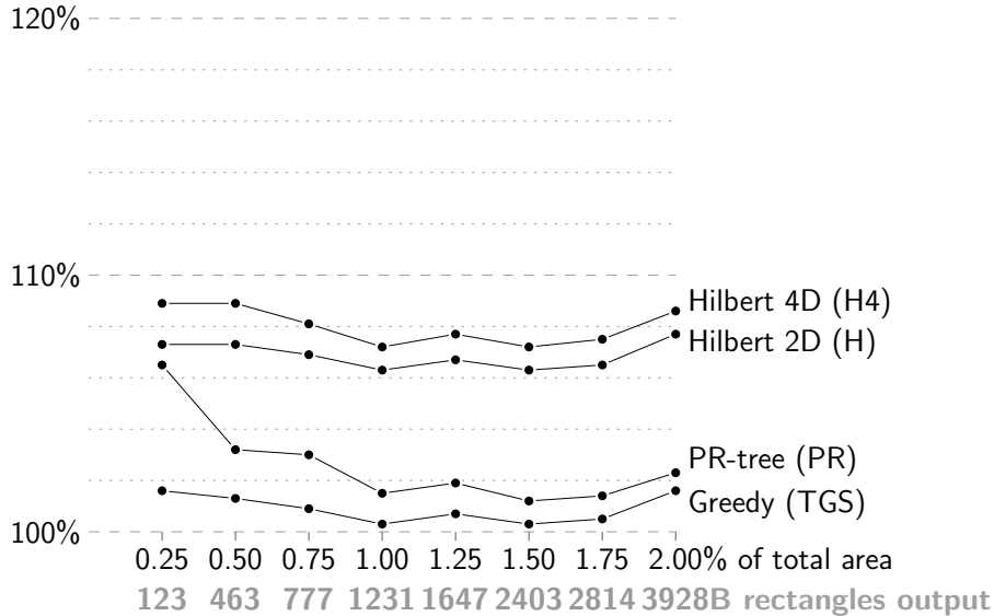
Fig. 12. Query performance for queries with squares of varying size on the Western TIGER data. The performance is given as the number of blocks read divided by the output size T/B .
