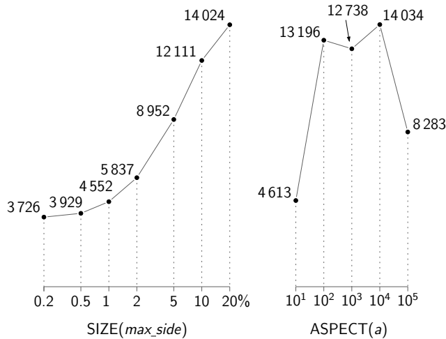
Fig. 11. Bulk-loading time in seconds of Top-down Greedy Split on synthetic data sets of 10 million rectangles each.
