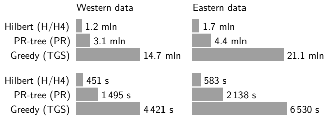
Fig. 9. Bulk-loading performance on TIGER data: I/O (upper figure) and time (lower figure).
