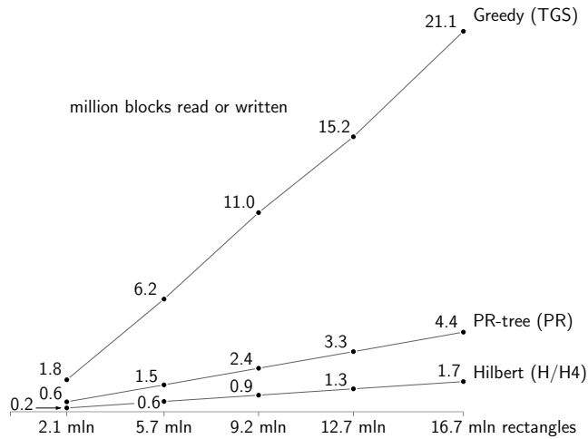
Fig. 10. Bulk-loading performances on Eastern datasets (I/Os)
