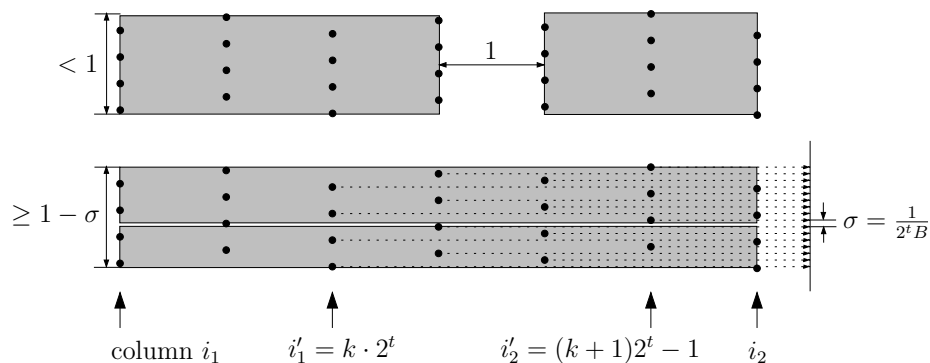
Fig. 4. TGS partitioning the worst-case example. A vertical division creates two bounding boxes with a total area of less than i_2 - i_1 - 1 . A horizontal division creates two bounding boxes with a total area of more than (i_2 - i_1)(1 - 2\sigma) > i_2 - i_1 - 1 .
