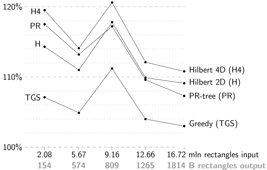
Fig. 14. Query performance for queries with squares of area 0.01 on Eastern TIGER data sets of varying size. The performance is given as the number of blocks read divided by the output size T/B .
