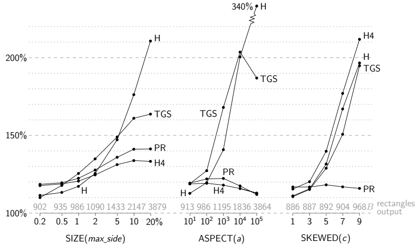
Fig. 15. Query performance for queries with squares of area 0.01 on synthetic data sets. The performance is given as the number of blocks read divided by the output size T/B .
