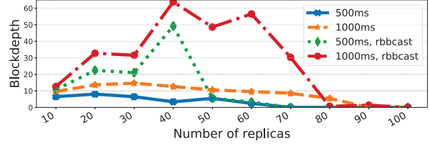
Fig. 6: Minimum finalization blockdepth m to obtain zero-loss for \mathfrak{D} = \mathfrak{G}/10 , f = \lfloor 5n/9 \rfloor - 1 .
