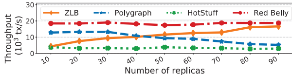
Fig. 3: Throughput of ZLB compared to that of Polygraph [18], HotStuff [79] and Redbelly Blockchain [25], [72].
