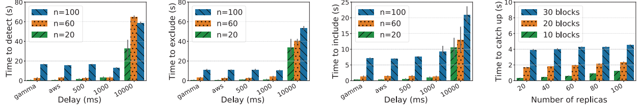
Fig. 5: (Left to right) Time to detect \lceil \frac{n}{3} \rceil a-b-c replicas, exclude them, include new replicas, per delay distribution and number of replicas; and catch up per number of blocks and replicas, with f = \lceil 5n/9 \rceil - 1 .
