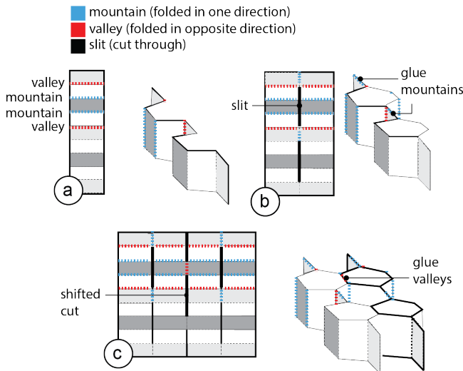
Figure 2: Folding honeycomb structures: (a) half a column of cells, (b) column of cells, (c) multiple columns.
