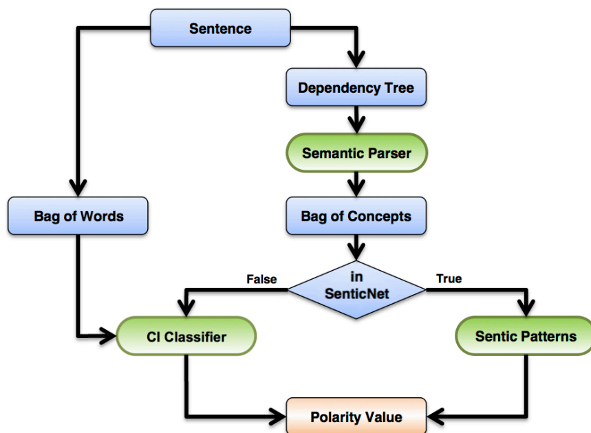
Figure 3: Sentence-level polarity detection algorithm. The semantic parser detects concepts in the text. The dynamic sentic patterns are applied to those concepts that are present in SenticNet, while other concepts are treated using statistical machine-learning methods.
