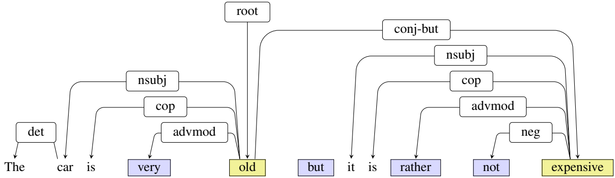
(a) Dependency tree of a sentence.
