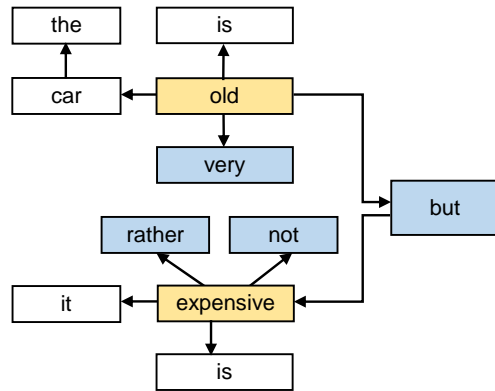
(d) The electronic circuit metaphor: sentiment words are “sources” while other words are “elements”, e.g., “very” is an amplifier, “not” is a logical complement, “rather” is a resistor, “but” is an OR-like element that gives preference to one of its inputs.
