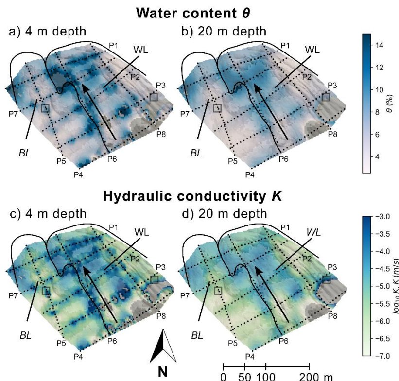
410 Figure 4: Water content (a and b) and hydraulic conductivity (c and d) visualized as slices parallel to the surface in two different depths. The edges of the black lobe (BL) and white lobe (WL) are indicated by black lines. Low sensitivity areas are displayed transparently, and the positions of electrodes are presented by black dots. Additionally, the direction of topography is indicated by a black arrow and the positions of tracer experiments by gray squares.
