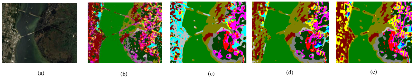
Fig. 10. KSC: (a) False color image, (b) to (e), classification maps for different classifiers: (b) EMP-SVM, (c) 3D-CNN, (d) 3D-GAN, (e) 3D-Aug-GAN
