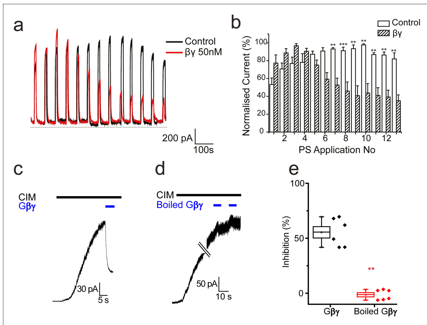
Figure 8. Effect of \beta\gamma subunits on PS-evoked currents. (a) Outward currents (+40 mV) evoked by 10 s PS (50 \mu M) applications every minute in TRPM3-expressing HEK293 cells. Cells dialysed intracellularly with \beta\gamma subunits (50 nM, red trace) showed a progressive decline in the evoked current amplitude compared to control cells. (b) Column graph displaying normalised current (% of maximum current) for PS-evoked outward currents in TRPM3-expressing HEK293 cells. Columns represent mean \pm SEM; ** p <0.01, *** p <0.001, unpaired t-test (control, n = 3–5 cells; \beta\gamma , n = 3–5 cells). (c) \beta\gamma subunits (50 nM) applied to the intracellular face of an inside out membrane patch from TRPM3-expressing HEK293 cell inhibit 10 \mu M CIM0216 evoked outward current (+60 mV). (d) Heat inactivated (100°C, 10 min) \beta\gamma subunits (50 nM) do not inhibit CIM0216 evoked currents in inside out membrane patches for \beta\gamma subunits ( n = 5) and boiled \beta\gamma subunits ( n = 6). ** p = 0.002
