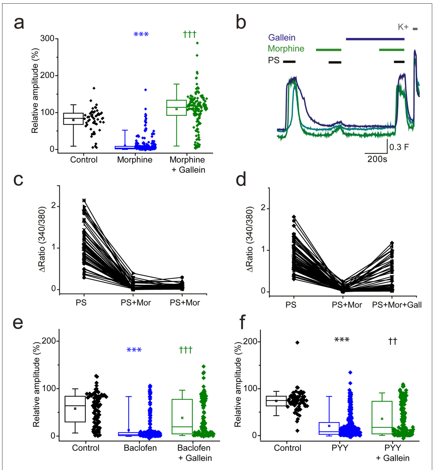
Figure 7. \beta\gamma subunits mediate G_{i/o} inhibition of TRPM3. (a, b) Effect of the G\beta\gamma inhibitor gallein (20 \mu\text{M} ) on morphine (10 \mu\text{M} ) induced inhibition of PS-evoked [\text{Ca}^{2+}]_i -responses. (a) Plots show the relative response amplitudes evoked by a second PS challenge (20 \mu\text{M} ) in control conditions, in the presence of morphine and gallein, control n = 52 ; morphine n = 314 ; morphine + gallein n = 153 . (b) Representative traces demonstrating that gallein reverses morphine inhibition of PS (20 \mu\text{M} ). Cells were perfused with 10 \mu\text{M} morphine 2 min before and during the second and third PS challenge, and perfused with 20 \mu\text{M} gallein 7 min before and during the third PS challenge. The results shown are for morphine sensitive cells (PS response amplitude in presence of morphine < 30% of the first response amplitude). *** p < 0.001 compared to control, ††† p < 0.001 compared to morphine, Kruskal Wallis. Figure 7 continued on next page
