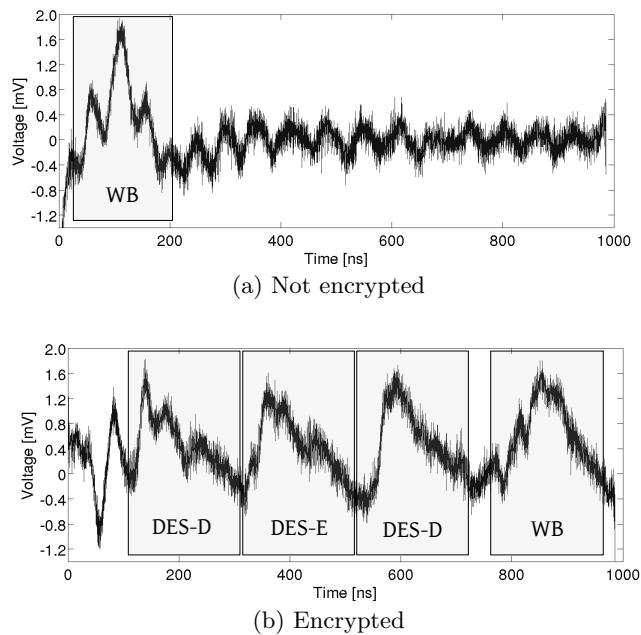
Figure 4: Filtered power consumption measured at VCC_{INT} during the time period of the decryption.
