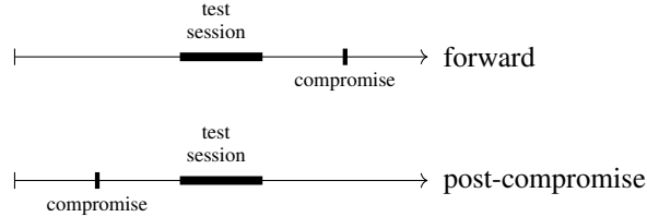
Figure 1: Attack scenarios considered by forward and post-compromise secrecy; “test” refers to the session under attack. Forward secrecy protects sessions against later compromise; Post-compromise secrecy protects sessions against earlier compromise.
