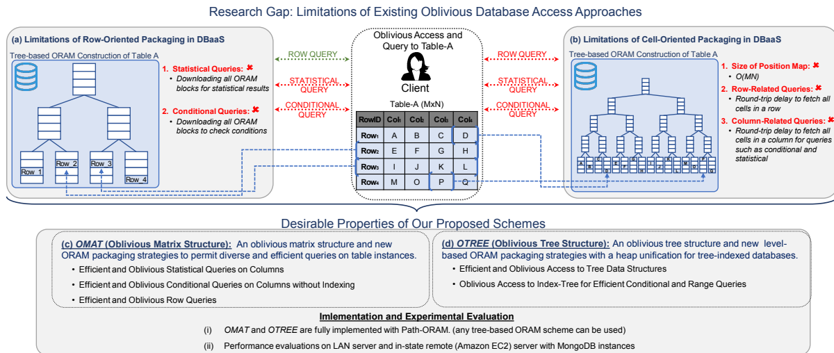
Figure 2. Research gap to be addressed and desirable properties of the proposed schemes.
