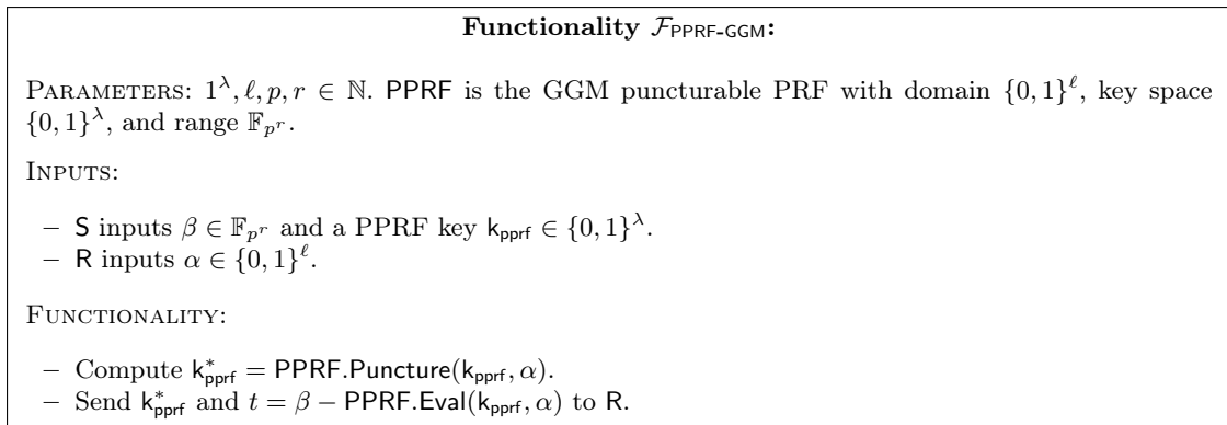
Fig. 5. Functionality for distributing a PPRF correlation
