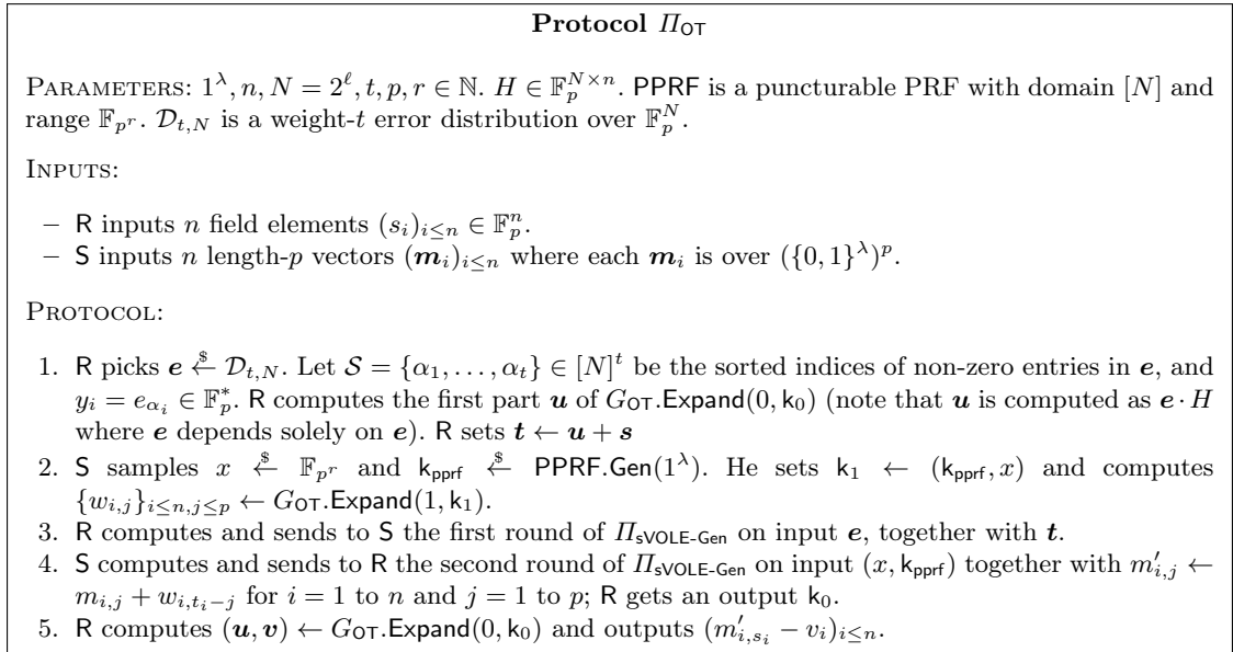
Fig. 10. Two-Round OT Extension
