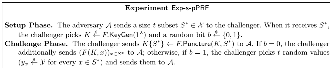
Fig. 1. Selective security game for puncturable pseudorandom functions. At the end of the experiment, \mathcal{A} sends a guess b' and wins if b' = b .
