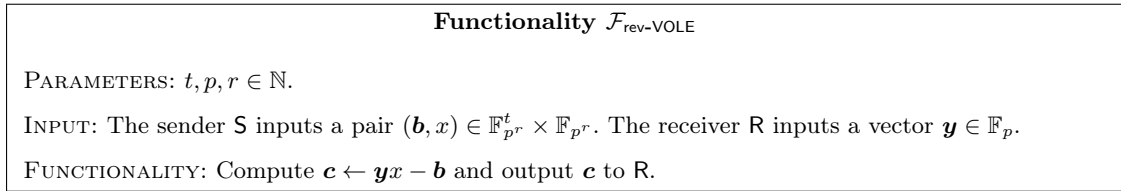
Fig. 8. Reverse Vector-OLE Functionality over a Field \mathbb{F}_p
