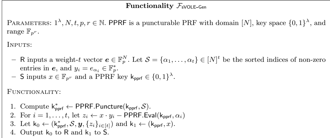
Fig. 7. Functionality for the Generation Procedure of the Subfield-VOLE Generator
