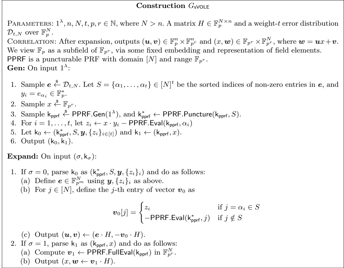
Fig. 3. PPRF-based PCG for subfield vector-OLE
