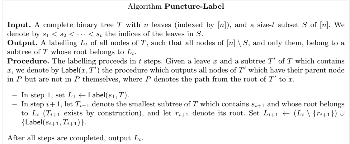
Fig. 18. Labelling algorithm to compute the indices of a subset of keys in the GGM PRF construction which allows to reconstruct the output of the GGM PRF at all points except exactly t .
