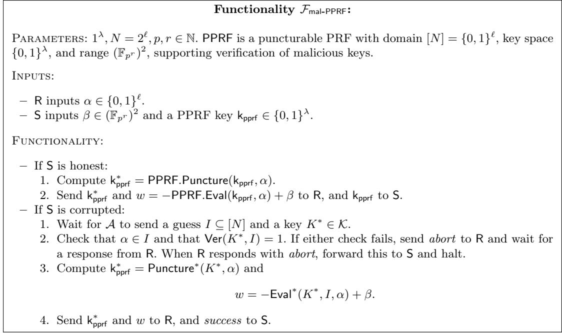
Fig. 12. Functionality for malicious distributed setup of single-point PPRF
