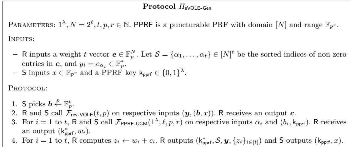
Fig. 9. Protocol for the Generation Procedure of the Subfield-VOLE Generator
