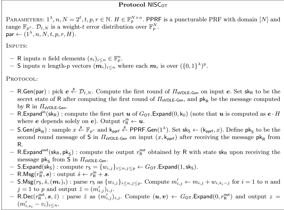
Fig. 11. Non-interactive secure computation with silent preprocessing for oblivious transfer
