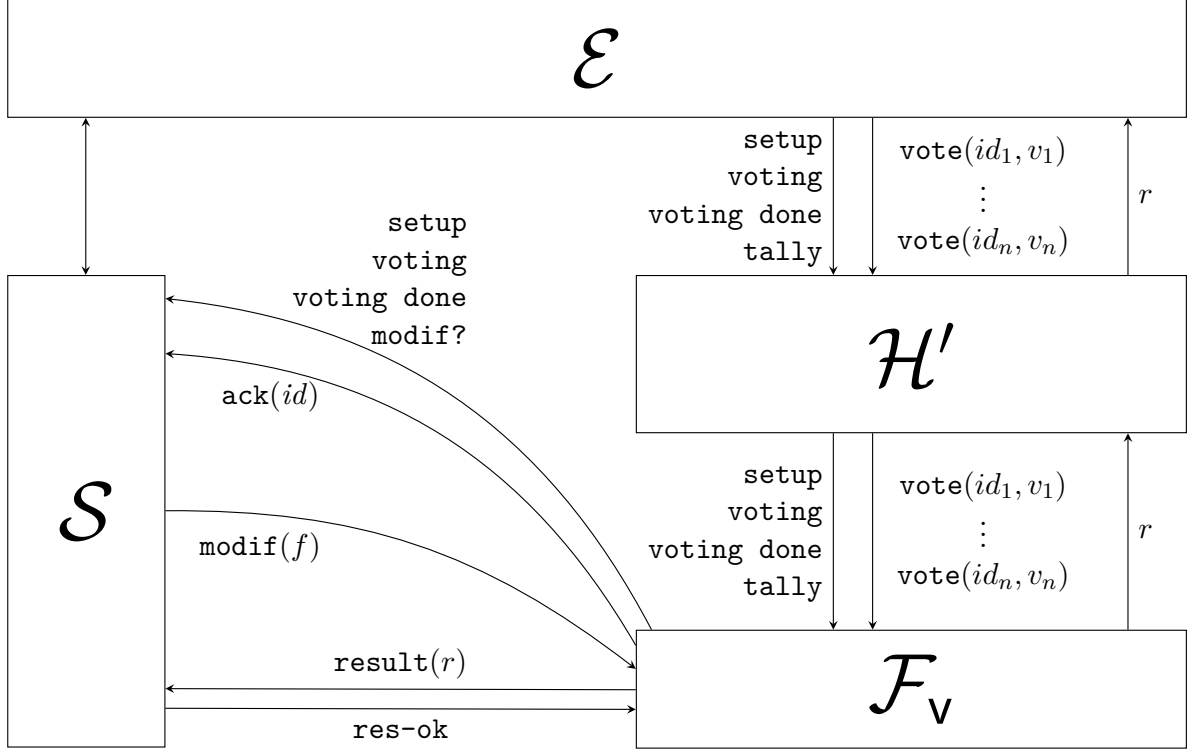
Figure 4: The ideal execution with id_1, \dots, id_n \in \mathsf{H}
