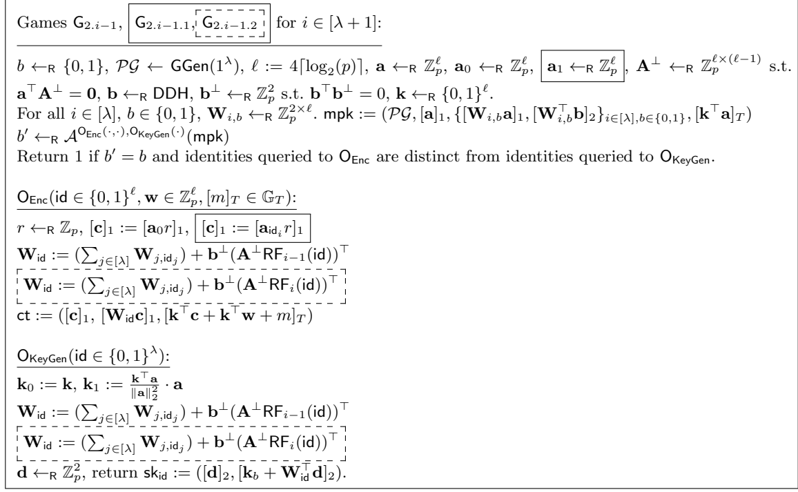
Fig. 10. Games for the proof of Lemma 3. In each procedure, the components inside a solid (dotted) frame are only present in the games marked by a solid (dotted) frame. Here, for all i \in [\lambda] , \text{RF}_i : \{0, 1\}^\lambda \rightarrow \mathbb{Z}_p^{\ell-1} denotes a random function that only reads the first i 'th bits of its input, and that is computed on the fly.
