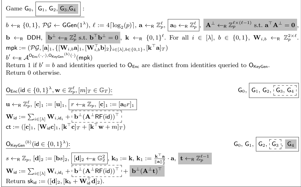
Fig. 9. Games for the proof of Property 2. In each procedure, the components inside a solid (dotted, gray) frame are only present in the games marked by a solid (dotted, gray) frame. Here, \text{RF} : \{0, 1\}^\lambda \rightarrow \mathbb{Z}_p^{\ell-1} denotes a random function that is computed on the fly.
