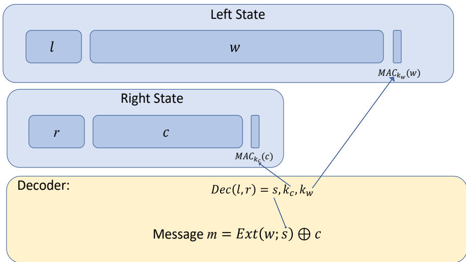
Figure 2: Overview of the construction. Blocks l, r come from augmented non-malleable code. The encoder proceeds in steps: first, we randomly sample s, k_w, k_c, w (all independently of the message we are encoding), then we encode s, k_w, k_c using NMC into l, r . We then set c = \text{Ext}(w; s) \oplus m , and evaluate \sigma_c as a MAC tag of c on key k_c , and \sigma_w as MAC tag of w on key k_w .
