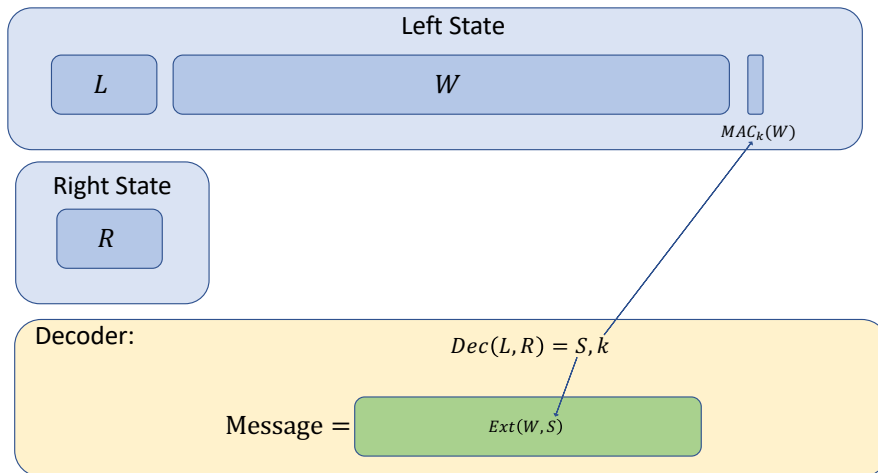
Figure 1: Construction of the non-malleable randomness encoder by [KOS18].
