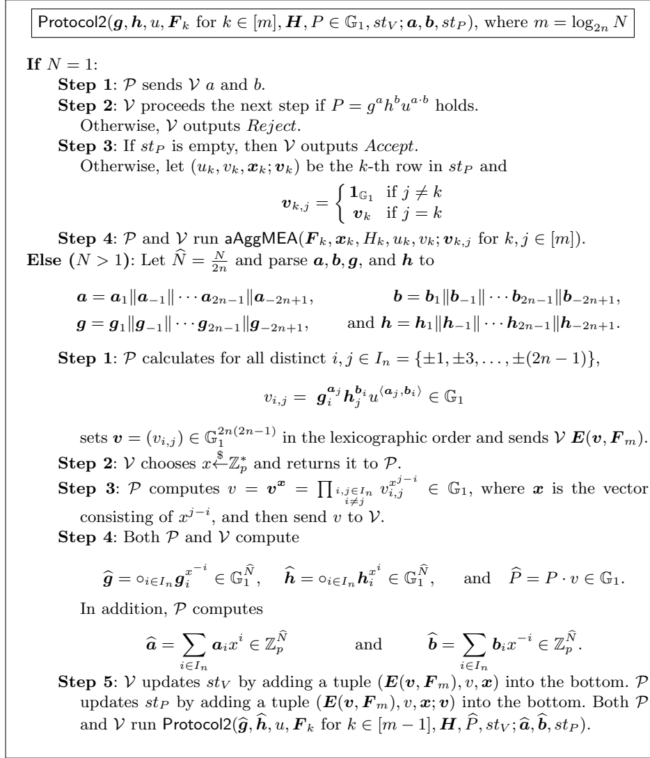
Fig. 3. Protocol2: Sublogarithmic IP Argument
