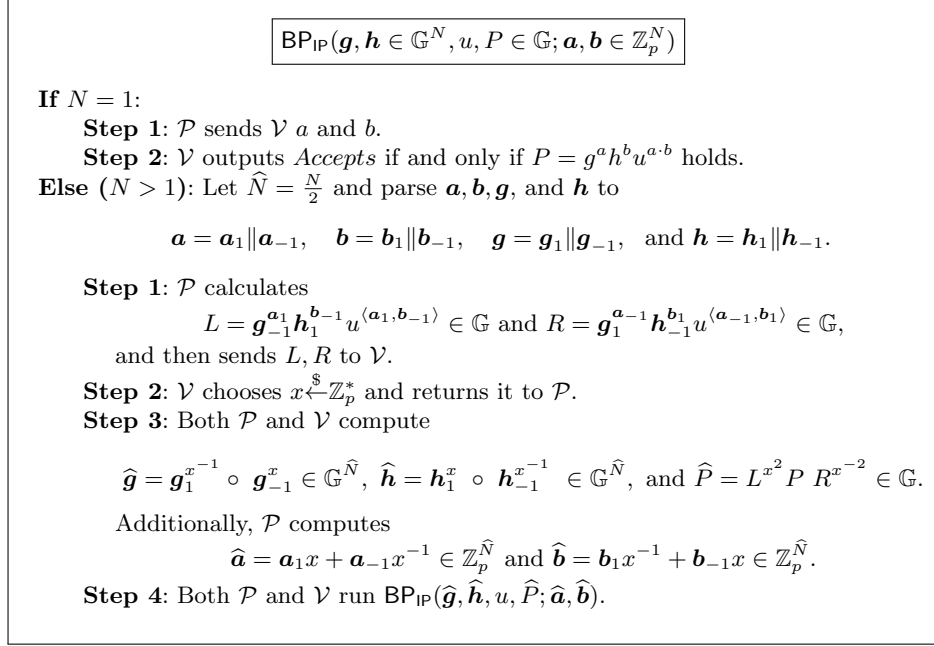
Fig. 6. Bulletproofs (Inner-Product Argument)
