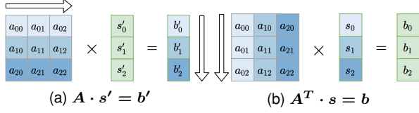
Fig. 1. Matrix-vector multiplication
