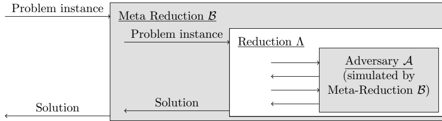
Figure 1: The meta-reduction technique of Coron [Cor02].
