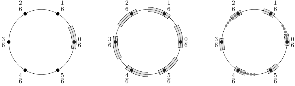
Figure 2: Visual heuristics for lemmata 3.8 and 3.9. The left figure is the intuition for lemma 3.8. The middle figure shows [0, K]_{\mathbb{Z}_p} + \mathbb{S}_6 + \mu . The right figure shows [0, K]_{\mathbb{Z}_p} + \mathbb{S}_6 + \mu and how points of the form ua/3 are distributed. Visibly, until the gray points first escape the intervals, they all lie within; after they escape, they never re-enter an interval. Hence at most 3 \cdot K/a points lie within [0, K]_{\mathbb{Z}_p} + \mathbb{S}_6 + \mu .
