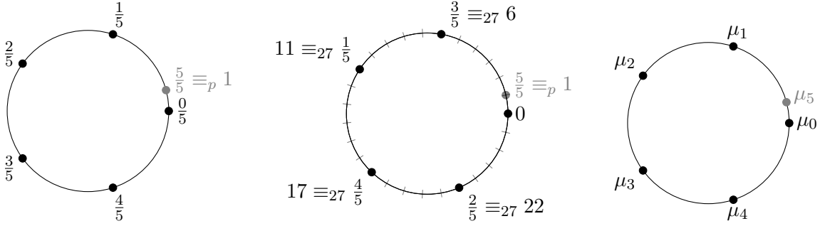
Figure 1: Visual heuristics for lemma 3.7. The left figure is the naive intuition. The middle figure is the visualization of for p = 27 . The right figure denotes \mathbb{S}_d = \{\mu_0, \dots, \mu_4\} where \mu_i \equiv_p \lceil \frac{ip}{d} \rceil . In the example, \mu_1 \equiv_{27} 6 , \mu_2 \equiv_{27} 11 , \mu_3 \equiv_{27} 17 , \mu_4 \equiv_{27} 22 .
