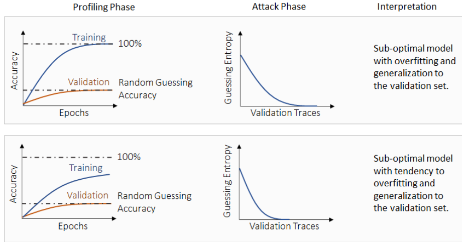
Fig. 2: Common model behaviors.
