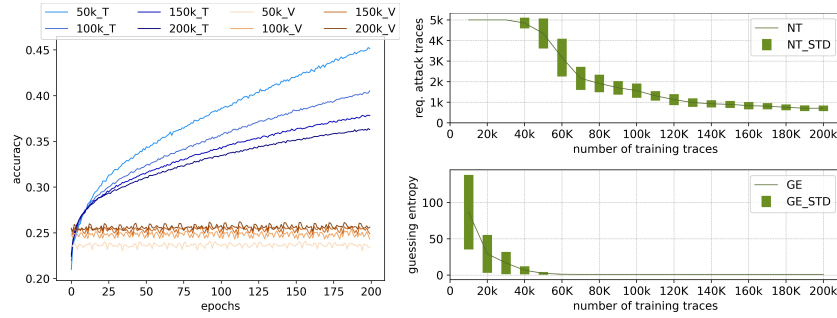
Fig. 4: Increasing the profiling set size and accuracy in the training (T) and validation (V) set and the required number of attack traces to reach GE = 1 , #8 in Table 1a.
