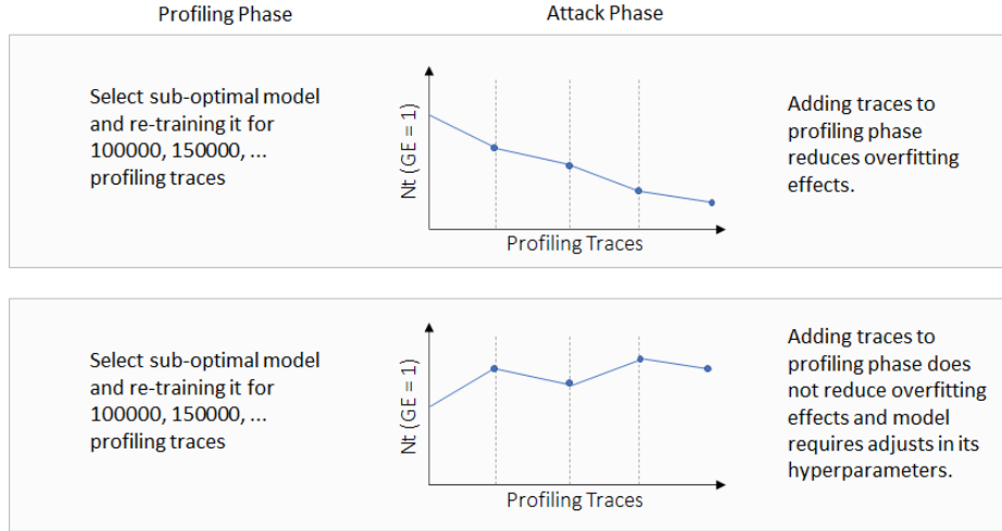
Fig. 3: Interpreting the model behaviors.
