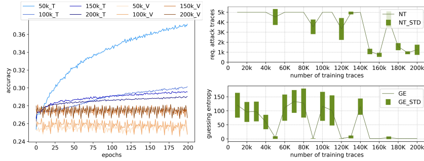
Fig. 5: Increasing the profiling set size and accuracy in the training (T) and validation (V) set and the required number of attack traces to reach GE = 1 , #2 in Table 1a.
