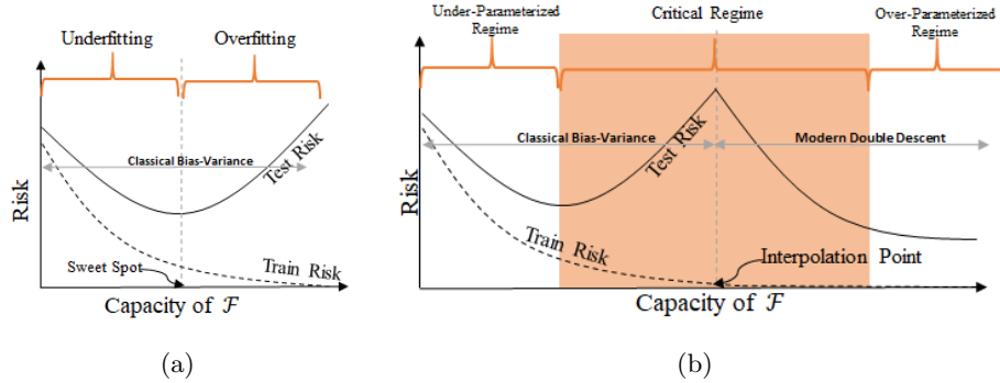
Fig. 1: Curves for training risk (dashed line) and test risk (solid line). (a) The classical U-shaped risk curve. (b) The Double Descent risk curve.
