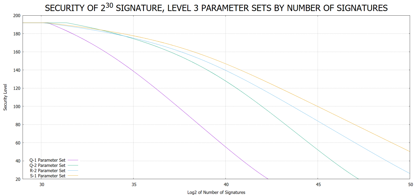
Figure 7: Recommended Parameter Sets for 2^{30} signature limit at level 3
