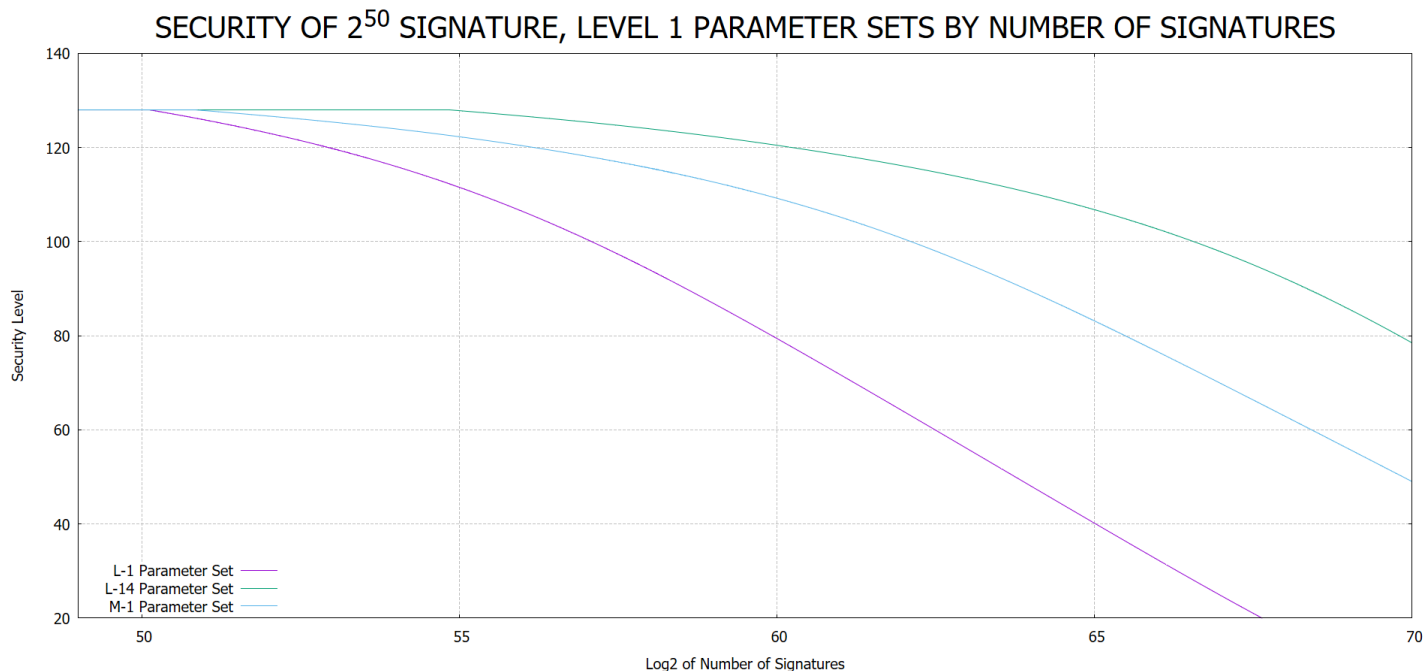
Figure 6: Recommended Parameter Sets for 2^{50} signature limit at level 1
