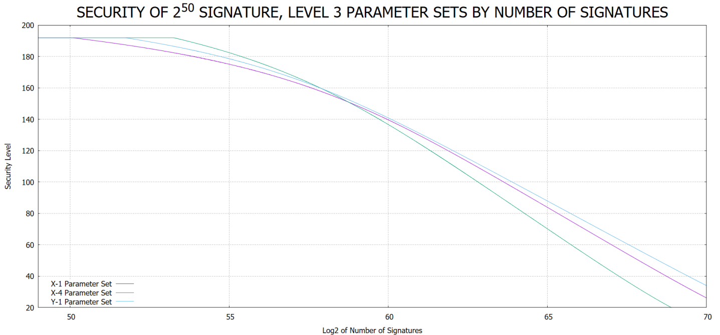
Figure 9: Recommended Parameter Sets for 2^{50} signature limit at level 3
