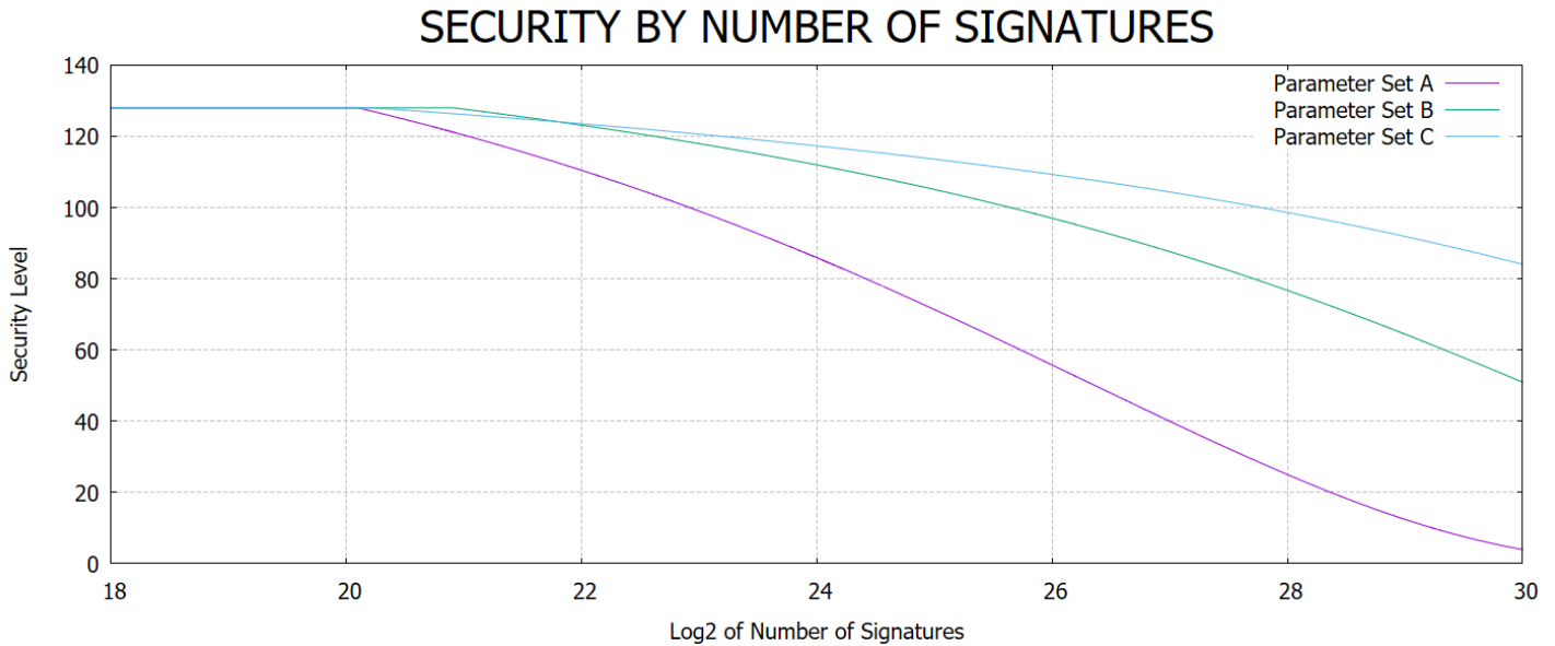
Figure 2: Overuse characteristics of the three example parameter sets
