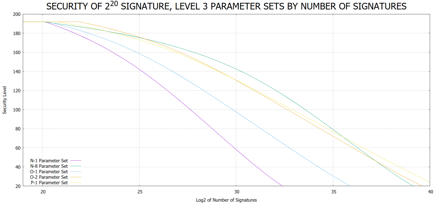
captionRecommended Parameter Sets for 2^{20} signature limit at level 3
