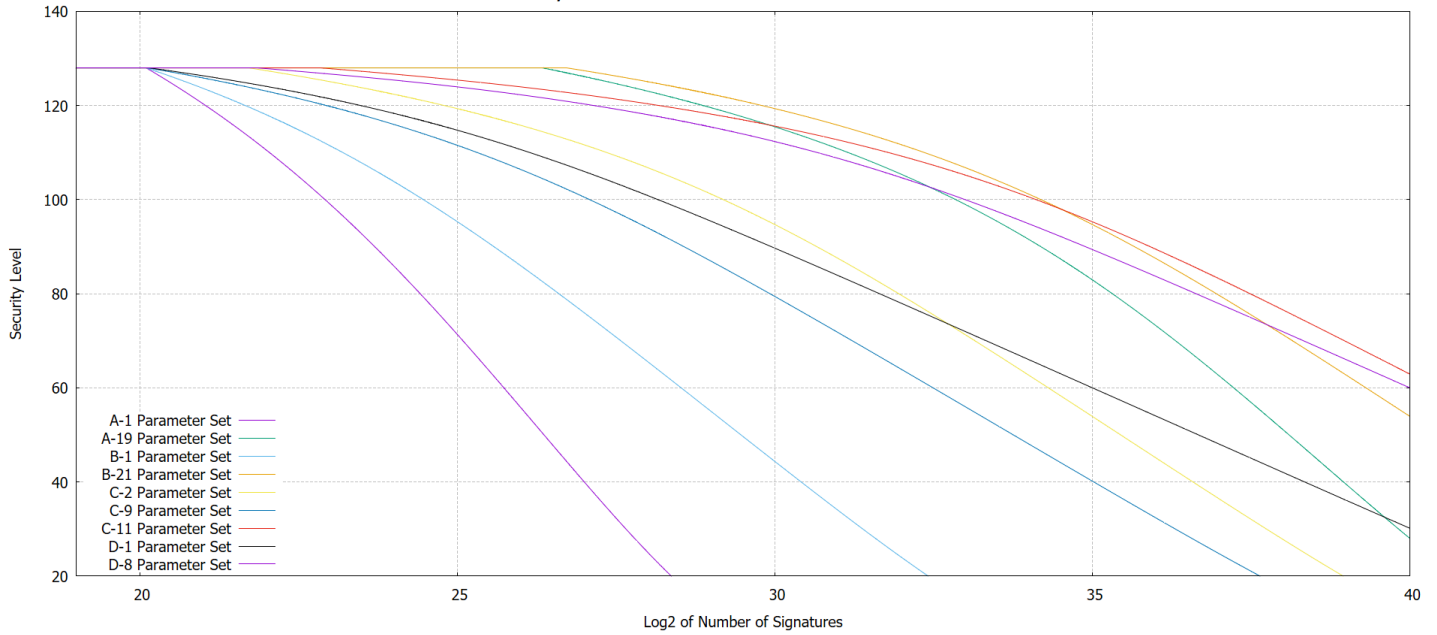
Figure 3: Recommended Parameter Sets for 2^{20} signature limit at level 1
