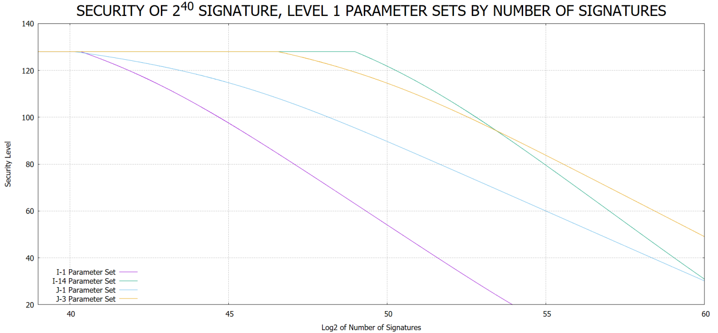
Figure 5: Recommended Parameter Sets for 2^{40} signature limit at level 1
