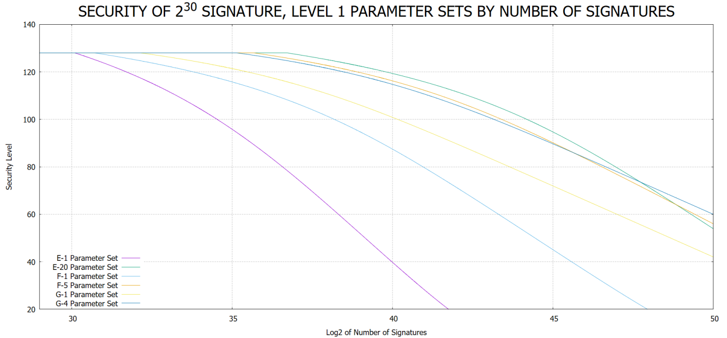
Figure 4: Recommended Parameter Sets for 2^{30} signature limit at level 1
