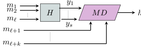
Figure 5: Linear Hash Mode H_2 using r + \lceil(s + k - 1)/(t - 1)\rceil many t -to-1 Compression Function Calls where MD is Merkle-Damgård hash function.
