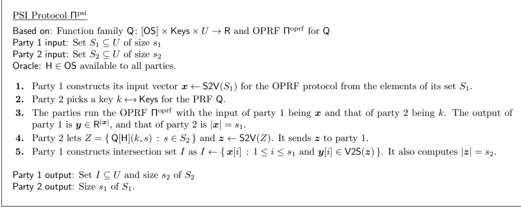
Figure 9: PSI protocol \Pi^{\text{psi}} associated to function family Q and OPRF \Pi^{\text{oprff}} for Q .
