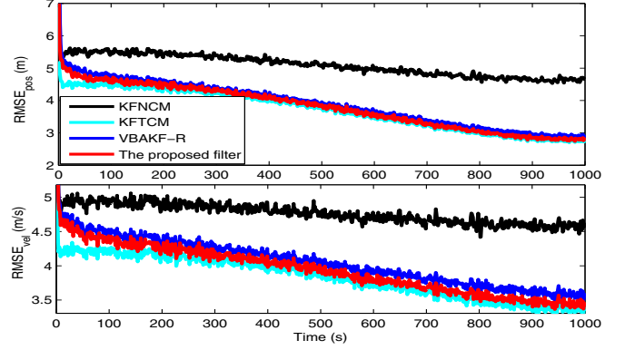
Fig. 9: RMSEs of the position and velocity when the nominal PNCM \tilde{\mathbf{Q}}_k and the true PNCM \mathbf{Q}_k are identical.
