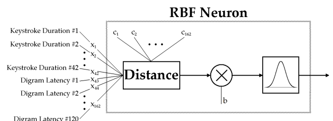
Fig. 1. The structure of the RBF neuron.
